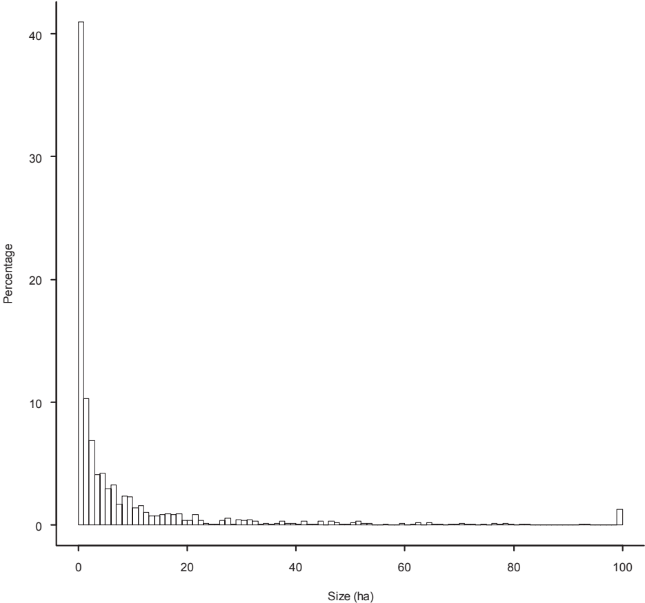
Figure B1. Distribution of the size of error ellipses for 22 VHF collared female red deer in Norway, in ha. All error ellipses larger than 100 ha ( n = 17 ) have been set to the size 100 ha. As the size was generally low (mean = 10.65 \pm 1.95 ha, median = 1.85 ha, range 0.00 - 675.66 ha), all locations were included in the analyses.
