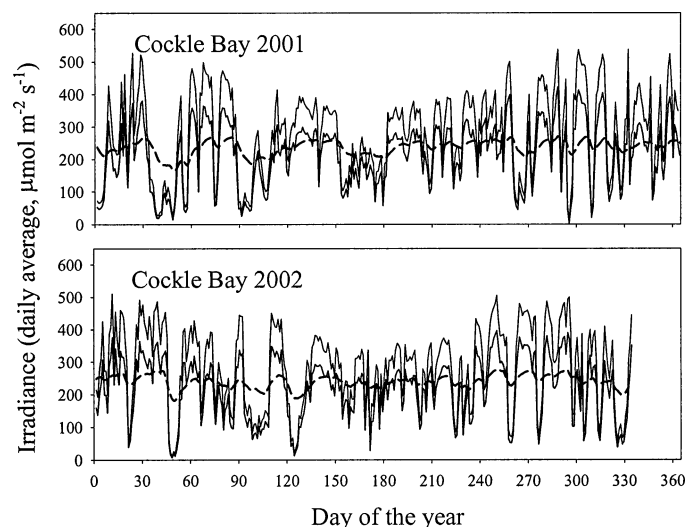
Fig. 6. Predicted benthic irradiance at 1.5 m below lowest astronomical tide (LAT) in Cockle Bay during 2001 and 2002. Data are upper and lower confidence limits (mean \pm 1 SD) of the average irradiance during the day ( \bar{E}(k_D, z) ) estimated with Eqs. 1 and 3. Confidence limits were estimated with the use of multivariate Monte Carlo analyses (see text). The dashed line indicates the predicted subsaturation constant ( E_k ) for the photosynthesis–irradiance response of the coral Turbinaria mesenterina with a 15% per day rate of photoacclimation (Anthony and Hoegh-Guldberg 2003; see also Web Appendix 1). Irradiances <E_k are suboptimal and indicate light-limited growth, and irradiances >E_k are supraoptimal, potentially leading to photoinhibition.
