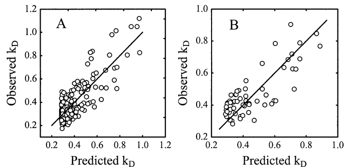
Fig. 5. Predicted versus observed attenuation coefficients ( k_D ) for the (A) model calibration using the first two data blocks ( n = 251 d), and (B) model evaluation with predictions based on the calibration and observed data from the third data block ( n = 63 d). In both cases, the residuals were normally distributed around the unity line, and the means and variances did not differ significantly between calibration and evaluation (see text for details).
