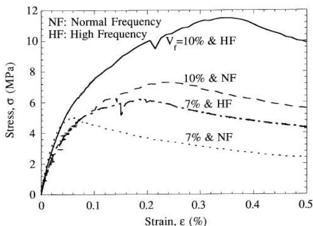
Fig. 5. Effect of vibration frequency during casting on tensile stress–strain curves for two different fiber volume fractions ( L_f = 6 mm).
