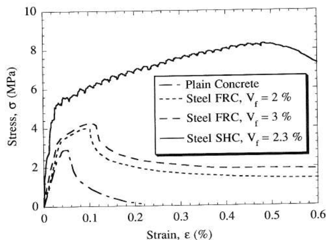
Fig. 7. Comparison between the tensile stress-strain response of strain-hardening cementitious composite (SHC, this study) and that of plain concrete and steel fiber reinforced concrete (after Soroushian and Bayasi 16 ).
