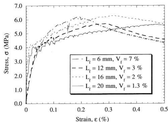
Fig. 4. Effect of fiber length (or aspect ratio) on tensile stress–strain behavior. Specimens cast under high-frequency vibration.
