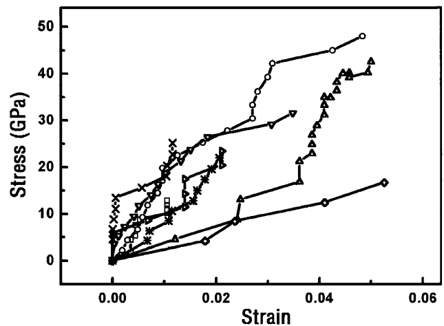
FIG. 2. Eight stress versus strain curves obtained from the tensile-loading experiments on individual SWCNT ropes. Each rope diameter is measured at high magnification ( \sim 100\,000 ) in the SEM, accuracy a few nm. The stress values have been calculated using the cross-sectional area of the perimeter SWCNTs, according to the geometric model [see Fig. 1(f) and Ref. [23]]. The SWCNT ropes for which strain could be determined were (see also Table I) C ( \square ), D ( \circ ), E ( \triangle ), G ( \nabla ), K ( \diamond ), M ( \triangleright ), O ( * ), P ( \times ).
