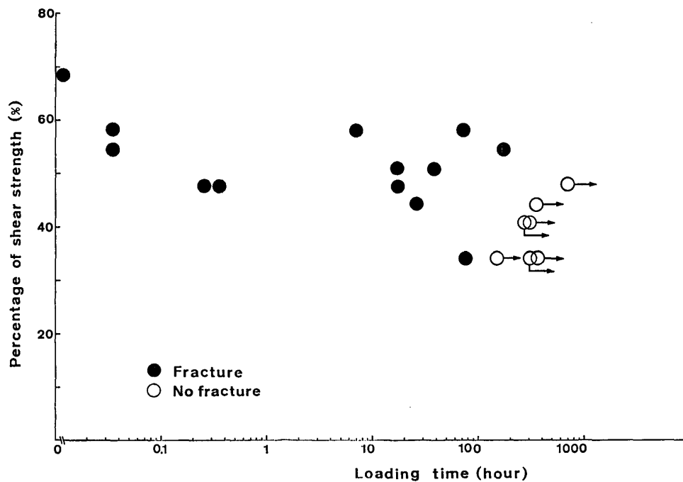
Fig. 6. Endurance curve.
