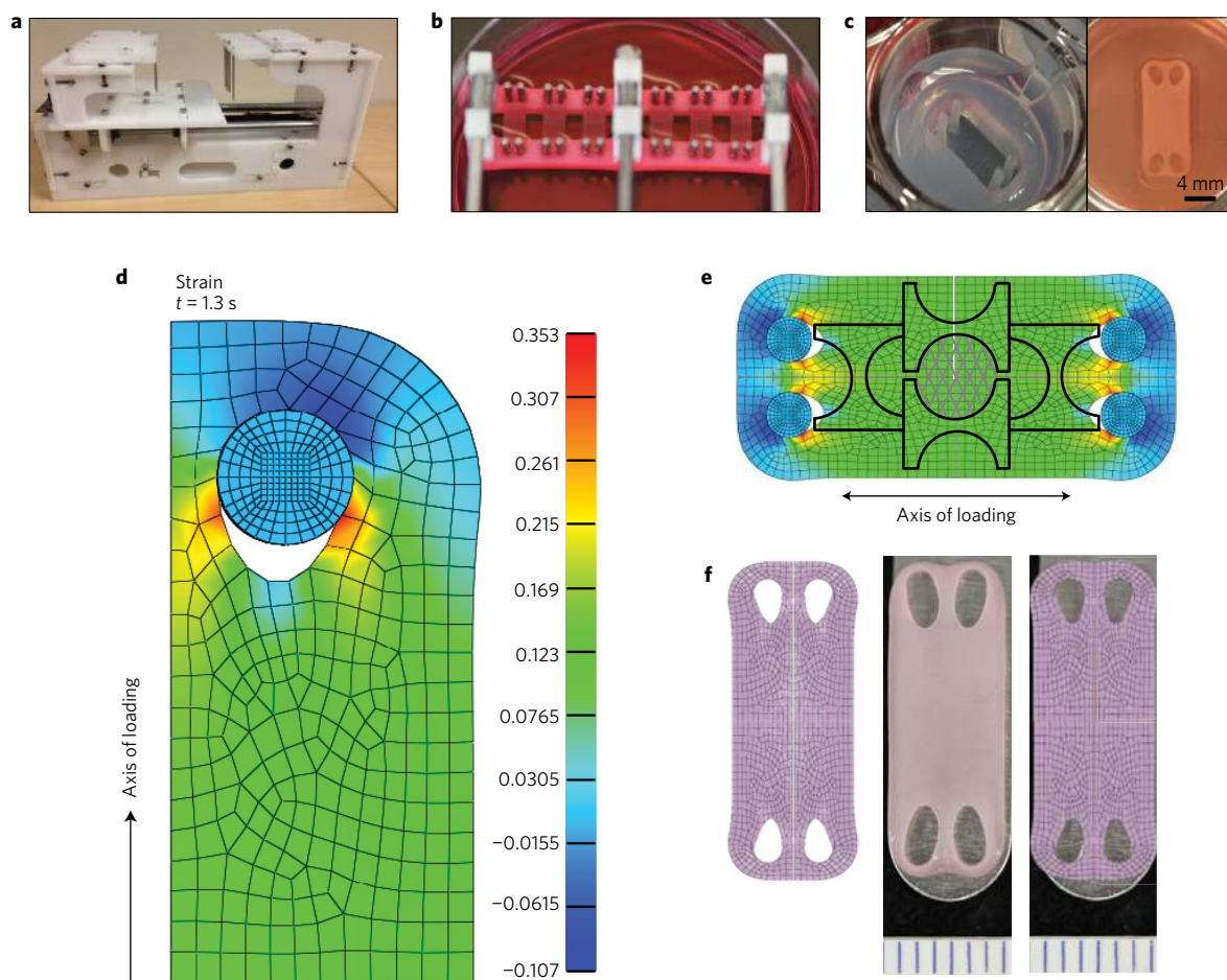
Figure 1 | Large-construct generation and uniform-strain validation. Modelling of stress and strain distribution during tension stimulation enabled the rational design of constructs displaying uniformity through the central portion. a , A custom tensile loading device was created for intermittent tension stimulation (InTenS). b , A custom tensile loading device was also designed and fabricated for continuous tension stimulation (CoTenS) of neocartilage. Tension stimulation was applied along the long axis. c , An agarose mould was created to generate rectangular self-assembled constructs. d , Modelling of stress and strain distribution during tension stimulation predicts uniform distribution through the centre of the neocartilage using a biphasic model. e , From the finite element model, uniform areas of strain were selected to portion compressive samples (hatched circle) and dumbbell-shaped parallel and perpendicular samples for tensile testing (outline). f , The finite element model was validated by overlaying the model with the actual deformed neocartilage.
