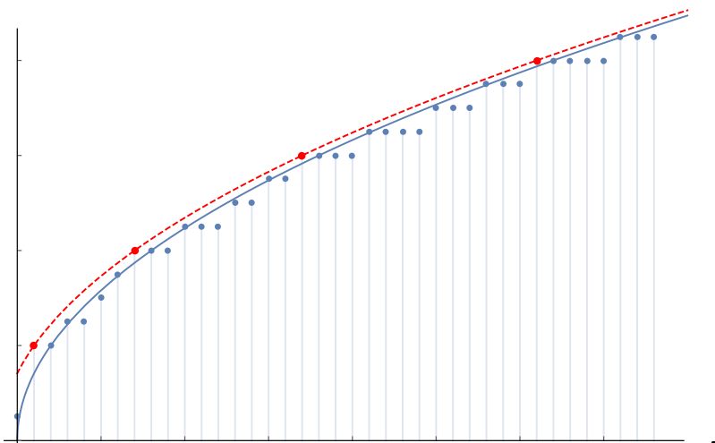
Figure 4. Maximal charge q_{\max}(n) for a \text{Bl}_1 \mathbb{P}^2_{112}[4] fibration over dP_2 , with (x, y_1, y_2) = (6, 2, 2) . The general features of this strongly coupled theory are completely in line with the findings of the previous examples, which correspond to weakly coupled strings.
