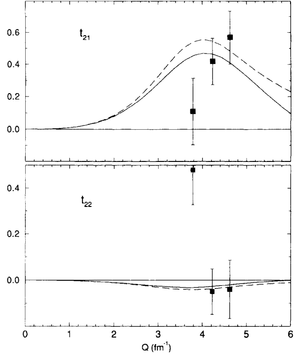
FIG. 11. t_{21} and t_{22} . Our data are not corrected for different electron angles (see Table II). The calculations were performed for \theta_e = 78.7^\circ using the form factors of Ref. [45], NRIA (dashed curve), NRIA+MEC+RC (solid curve).
