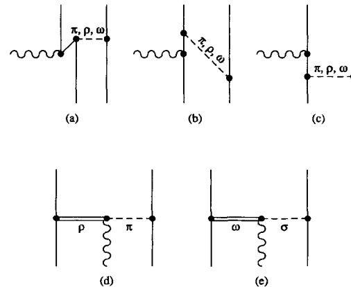
FIG. 9. Meson exchange diagrams: (a) pair term, (b) recoil, (c) reorthonormalization, (d) \rho\pi\gamma , (e) \omega\sigma\gamma (so far taken into consideration only in Refs. [66,66,71]).
