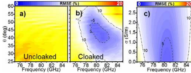
Fig. 6. RMSE distribution vs. incident angle and frequency for (a) uncloaked, and (b) cloaked bump. (c) RMSE distribution as a function of the conductivity \sigma of dielectric substrate and frequency.
