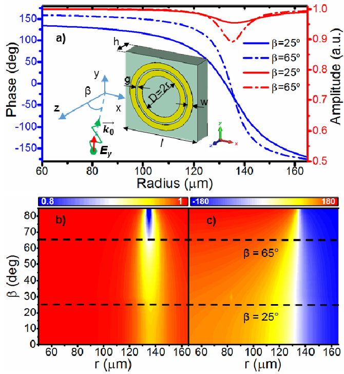
Fig. 2. (a) Phase response of the unit cell for different angles of incidence. (Inset indicates the unit cell geometry and its corresponding parameters. Color-map for the (b) amplitude and the (c) phase of the reflection coefficient as a function of the incidence angle and radius of the inner ring.
