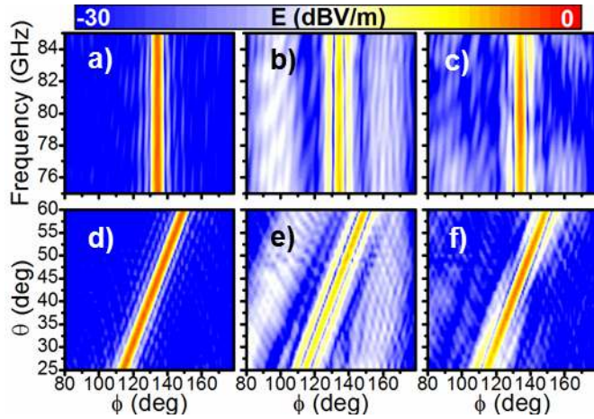
Fig. 5. Amplitude of the far-field component of the electric field as a function of azimuth angle \phi and frequency (a-c) and as a function of the incidence angle \theta and azimuth angle \phi (d-f). Left column refers to the beam reflected from the ground plane, center from the bare bump and right column the recovered the beam.
