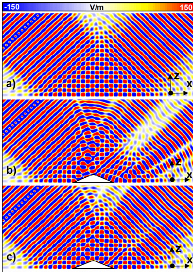
Fig. 3. Electric field distribution on xz -plane for (a) ground plane, (b) bare bump and (c) cloaked bump.
