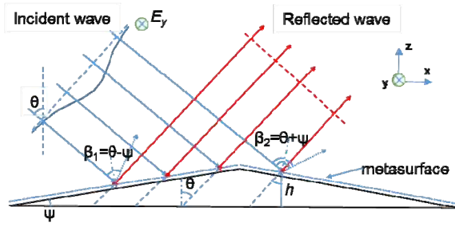
Fig. 1. A scheme of the carpet cloak with metasurface.
