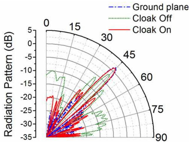
Fig. 4. Radiation pattern for the reflected Gaussian beam from the ground plane (dash-dotted blue line), the bump without cloak (dotted green line) and from the cloaked bump (solid red line).
