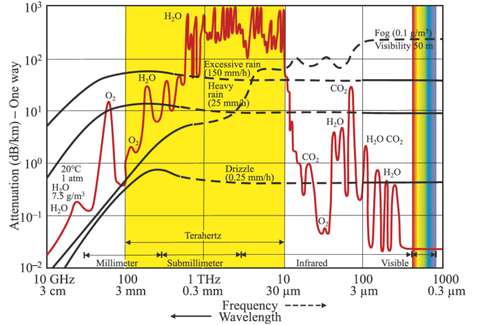
Fig. 1. Comparison between the attenuation impact of different environmental effects on different technologies [28].
