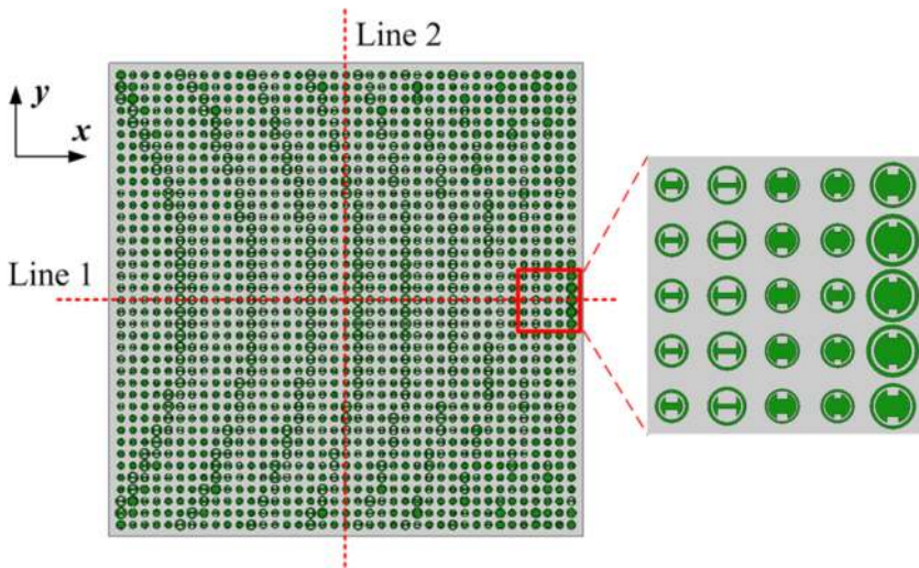
Fig. 11 Element arrangement of the THz transmitting and reflective metasurface. Reproduced from [136] under Creative Commons Attribution 4.0 International License ( https://creativecommons.org/licenses/by/4.0/ )—part of the whole original figure
