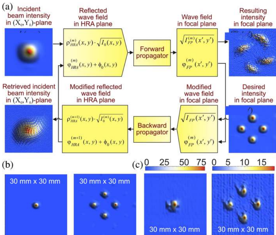
Fig. 9 a The work-flow of the Gerchberg-Saxton iterative algorithm for retrieving surface distribution. b, c Focusing performance of the holographic metasurface. Theoretical ( b ) and experimentally measured ( c ) intensity distributions in the focal plane at the frequency of 0.35 THz forming one and four focal spots, respectively. Reproduced from [117] under Creative Commons Attribution 4.0 International License ( https://creativecommons.org/licenses/by/4.0/ )—Fig. 2 from original article has shortened caption, parts of Fig. 6 are used with rephrased caption
