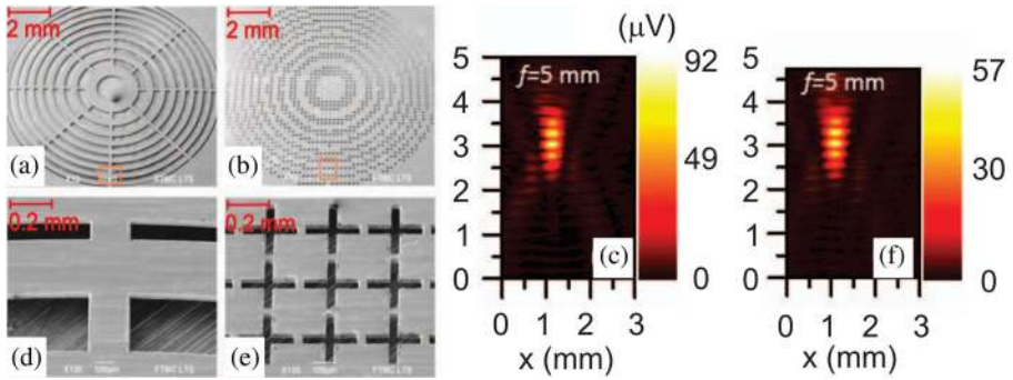
Fig. 6 The SEM images of the diffractive optical components with the focal length of 5 mm and the diameter of 16.5 mm. a The Fresnel zone plate and b the terahertz zone plate (TZP) both processed on metal film. d , e correspond to magnified regions marked in a and b with red rectangles. Images of the THz beam focused with the conventional zone plate ( c ) and the TZP ( f ). Pixel size 25 \times 25 \mu\text{m}^2 . © 2015 IEEE. Reprinted, with permission, from Minkevičius et al. [77]
