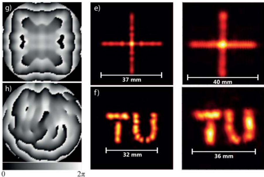
Fig. 10 Calculated phase modulation profiles (left). Calculated intensity distributions (middle) after the last iteration step of the GS algorithm. Experimental intensity distributions (right) of the optical field produced by an incident THz beam that was phase modulated by the two printed elements. Reproduced from: Gospodaric, J., Kuzmenko, A., Pimenov, A., Huber, C., Suess, D., Rotter, S., Pimenov, A.: 3d-printed phase waveplates for THz beam shaping. Applied Physics Letters 112(22), 221104 (2018), https://doi.org/10.1063/1.5027179 , gospodaric20183d , with the permission of AIP Publishing and author
