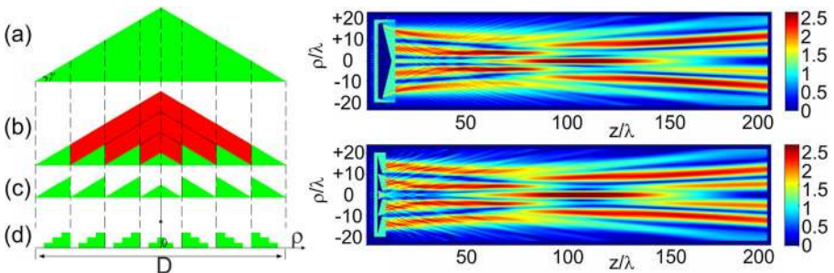
Fig. 8 (left) The design process of a diffractive axicon. a A bulk axicon. b An axicon with removed unwanted material (red part). c An equivalent kinoform axicon. d An equivalent 4-level phase axicon. (right) Electric-field amplitude patterns plotted in a pseudo-color representation: (upper) for the bulk axicon, (lower) for designed axicon ( d ). Reproduced from [104]
