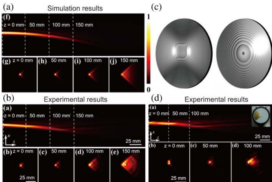
Fig. 7 Simulation (a) and experimental (b) results of the finite-energy accelerating THz airy beam. The upper row indicates the xz -normalized intensity profiles of the airy beam. The lower row indicates the xy -normalized intensity profiles of the experimentally generated airy beam measured at the dash line positions of the upper image. c Profiles of two elements creating airy beam. Additionally, experimental results of airy beam creation for “damaged” lens are shown (d). Reproduced from [101]
