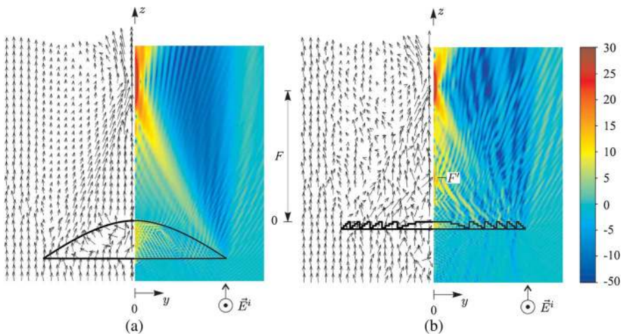
Fig. 4 Magnitude and direction of the time average of the Poynting vector—comparison of hyperbolic lens (a) with phase correcting zone plate (b), having the same focal lengths and diameters. © 2007 IEEE. Reprinted, with permission, from Reid et al. [46]
