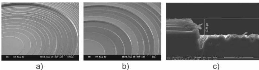
Fig. 5 SEM images tilted at 60 deg of a 16-level and b 4-level lenses and c cleaved lens fragment. © 2013 IEEE. Reprinted, with permission, from Saha et al. [64]. Reproduced from Komlenok et al. [68]
