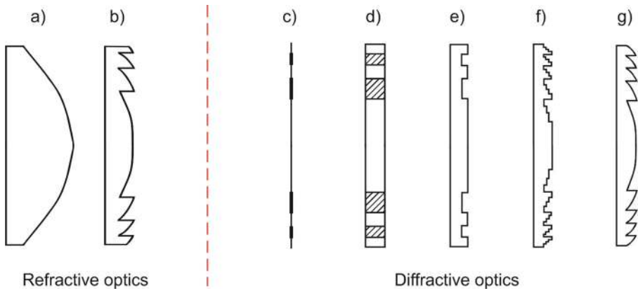
Fig. 3 Refractive (a, b) and diffractive (c–g) lenses. a Bulk lens. b Fresnel lens (not used in the THz range of radiation). c Fresnel zone plate—amplitude binary. d Planar dielectric zone plate—structure created from two materials with different refractive indices that corresponds to phase binary grating. e Binary phase—phase-reversing zone plate. f Multi-level zone plate. g Kinoform (Fresnel diffractive lens). Defined in Table 1. Adapted on the basis of [45]
