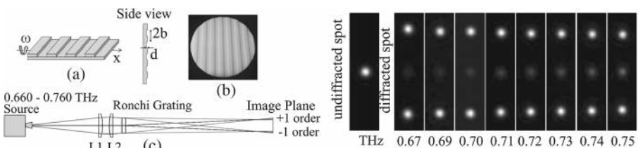
Fig. 1 a Grating design. b Photograph. c Optical far-field configuration. (right) Measured THz spots showing the frequency-dependent evolution of the -1 , 0 , and +1 diffracted orders. Reproduced from [34]
