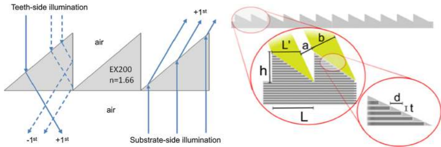
Fig. 2 Explanation of shadow effect based on geometrical optics, considering illumination from both sides (left) and at some angle (right). Dashed rays are misdirected into -1st order by the shadow effect. (right) ©2016 IEEE. Reprinted, with permission, from Busch et al. [38]. (left) Reproduced from Suszek et al. [39]
