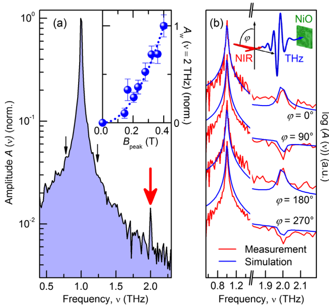
FIG. 3. (a) Normalized spectrum of the magneto-optical signal for B_{\text{peak}} = 0.4 T [see Fig. 1(d), top curve] extracted for delay times t > 4 ps. The sharp Lorentzian peak at 1 THz results from the long-lived oscillation of the 1-THz magnon mode. Surprisingly, an additional peak is found at the second harmonic frequency \nu = 2.0 THz. Black arrows: spectral positions of sum- and difference-frequency components of the 1 and 0.23-THz magnon mode. Inset: Spectral weight A_w of the peak at \nu = 2.0 THz as a function of the THz driving field B_{\text{peak}} (blue spheres, experimental data; dotted line, quadratic fit). (b) Magnon spectra induced by THz peak fields of 0.4 T for various angles \varphi of the probe polarization with respect to the crystal lattice (red curves, experimental data; blue curves, simulation).
