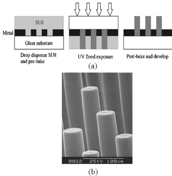
FIG. 1. SU8 pillar arrays, showing (a) fabrication flow on silicon substrates, and (b) final device realization.
