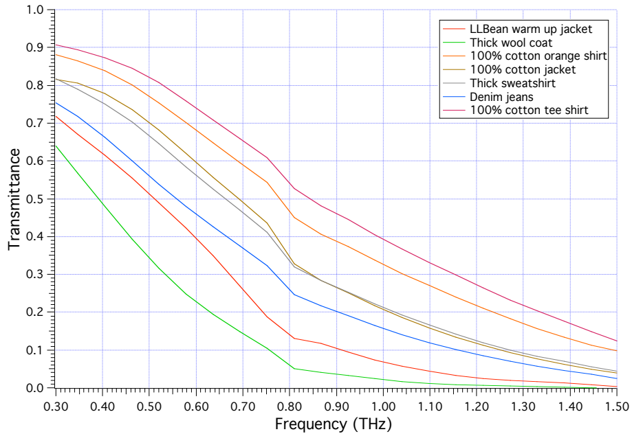
Figure 4.1. Plot of transmission through common clothing materials over terahertz frequencies from 0.3 THz to 1.5 THz. Apparent feature at 800 GHz for all samples is a spectrometer artifact.
