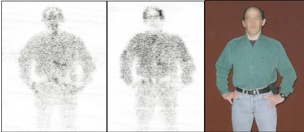
Figure 6.3. 1.56THz co-pol receive(VV) on left, and cross-pol receive (VH) in center. Photograph of the subject is on the right.
