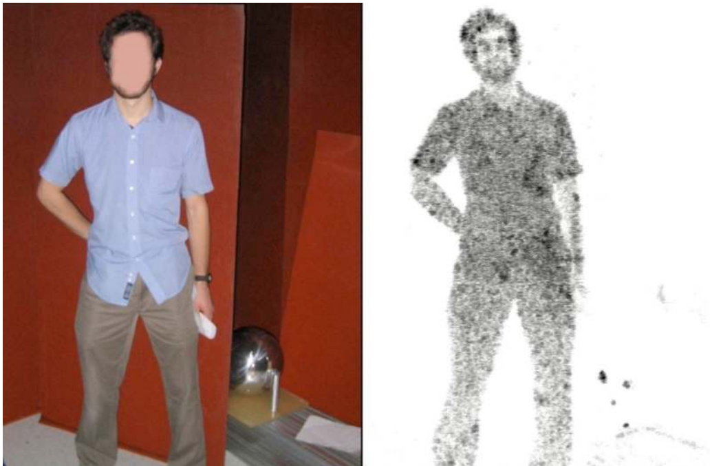
Figure 6.2. Imagery collected using the prototype, active illumination, CW, 1.56 terahertz system on the right. Spot size is approximately 6 millimeters. On the left is a photograph of the subject taken immediately following the scan. A concealed weapon can be seen in the subject's left breast pocket (reader's right). Polarization is cross-pol (VH).
