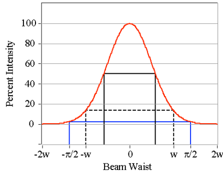
Figure 5.3. A Gaussian beam intensity profile, showing beam width definitions FWHM (black) , 1/e^2 (dotted), and \pi\omega (blue).
