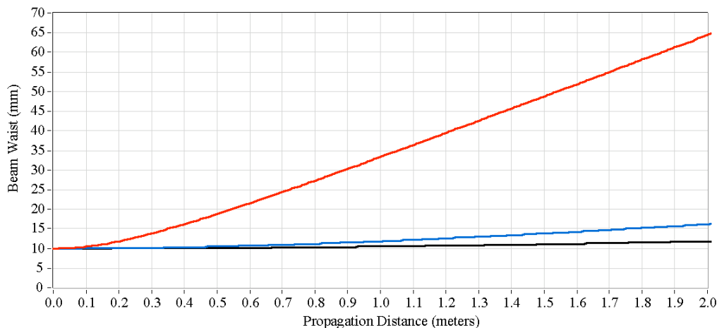
Figure 5.2. Initial Gaussian beam waist size of 10mm, propagated over 2 meters, for three frequencies, 0.3THz (red, upper), 1.5THz (blue, middle), and 3THz (black, lower).
