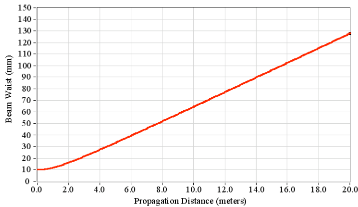
Figure 5.4. 1.56THz Gaussian beam waist size starting at 10mm, propagating 20 meters.
