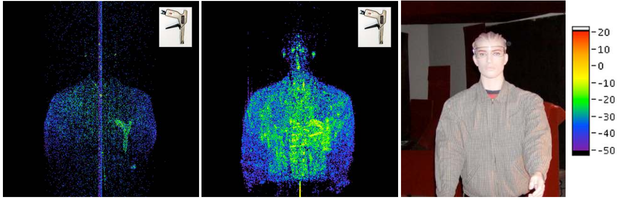
Figure 3.1. Azimuth/elevation collection of a clothed mannequin with a concealed, metal tie-wrap "gun"(inset). Left image taken at 1.56THz. Center image taken at 350GHz (dBV 2 color scale). Photograph of subject as measured on right. Note the penetration through the black plastic wrapping of the trigger handle at 350GHz. The black plastic wrap is heavily attenuating at 1.56THz and minimally attenuating at 350GHz, allowing the handle metal to reflect brightly.
