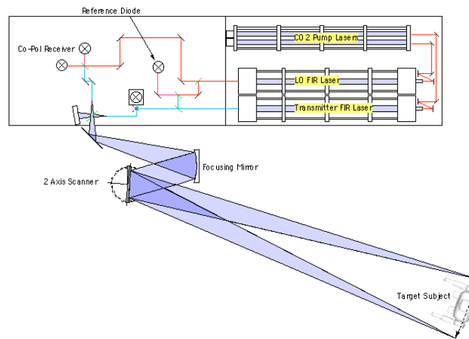
Figure 5.5. An overview of the optical design, showing relative locations of the monostatic transmitter/receiver, focusing mirror, two-axis scan mirror, and the target subject, initially a mannequin.
