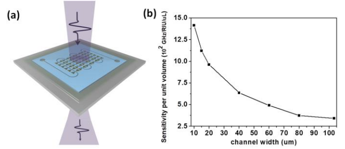
FIG.2. (a) Schematic diagram of the proposed device based on a bow-tie array MM. (b) Simulated sensitivity per unit volume for different channel widths based on a bow-tie array MM.
