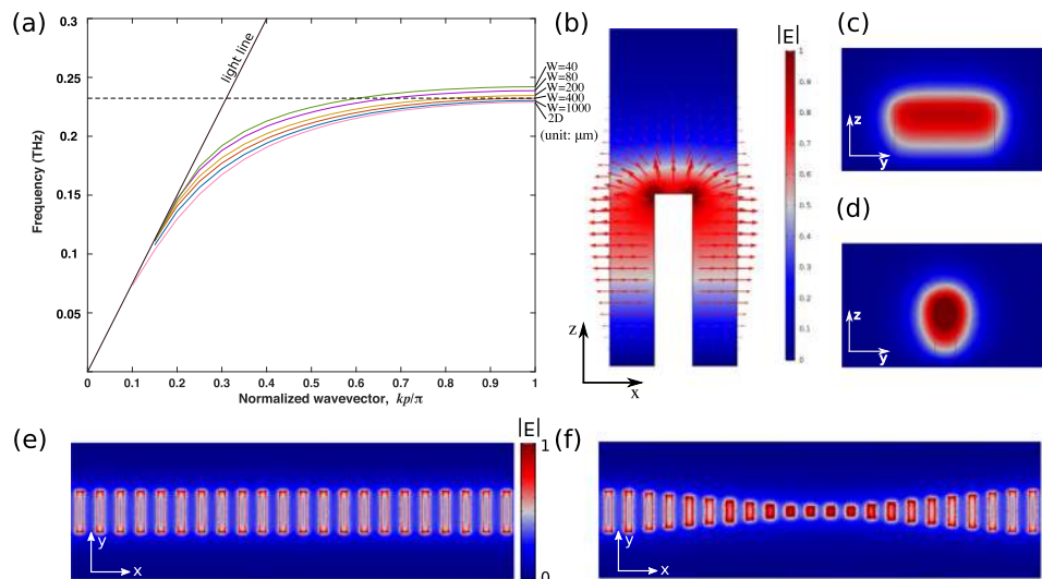
FIG. 2. (a) Dispersion curve of the spoof SPP modes for domino blocks with different lateral widths W = 40 \mu\text{m} , 80 \mu\text{m} , 200 \mu\text{m} , 400 \mu\text{m} , and 1000 \mu\text{m} , with other geometrical parameters fixed as p = 200 \mu\text{m} , h = 270 \mu\text{m} , and g = 140 \mu\text{m} . The 2D line corresponds to infinitely wide domino ( W \rightarrow \infty ), and the light line is indicated with a solid black line. The dashed line marks the cutoff frequency of the spoof SPP for W = 400 \mu\text{m} . The normalized electric field distribution of the spoof SPP wave from (b) xz -plane and yz -plane with (c) W = 400 \mu\text{m} and (d) W = 80 \mu\text{m} . Normalized electric intensity at the plane of the domino top for (e) the homogeneous waveguide and (f) the tapered waveguide. The width of the homogeneous domino waveguide is W = 400 \mu\text{m} , for the tapered waveguide, the domino blocks start from W = 400 \mu\text{m} and decrease in 40 \mu\text{m} step to W = 80 \mu\text{m} .
