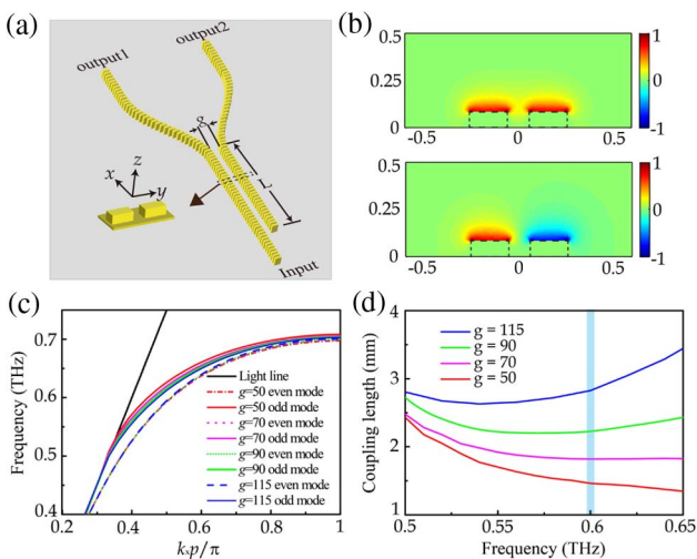
Fig. 4. (a) Schematic of the DC with relevant parameters. (b) Normalized electric component ( E_z ) distribution for the yz cross section of even (upper) and odd modes (lower) supported by two parallel waveguides. (c) Dispersion relation of even and odd modes for DCs with varying g . (d) Calculated coupling length for DCs with different g values of 115, 90, 70, and 50 \mu\text{m} .
