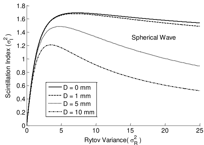
Figure 4.8 Scintillation index of a spherical wave vs. Rytov variance with different aperture diameters. (wavelength 1550nm, L = 1 km).
