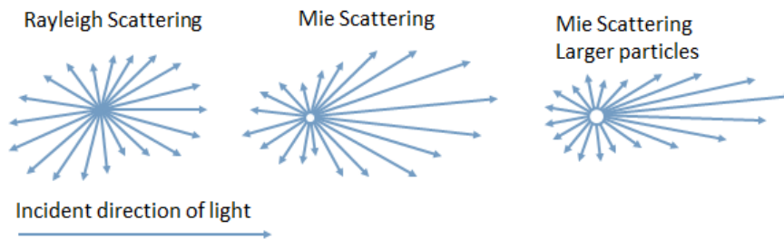
Figure 2.9 Rayleigh and Mie scattering. Source: [77]
