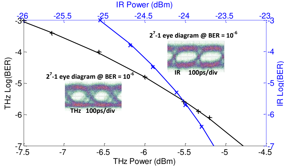
Figure 7.6 Sensitivity curves of THz and IR links. Inset: Eye diagrams of THz and IR signals at \text{BER} = 10^{-6} .
