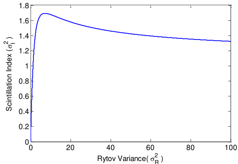
Figure 4.6 Scintillation index vs. Rytov variance for spherical wave.
