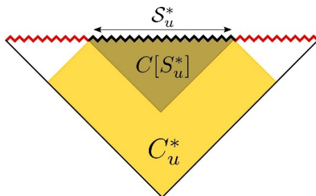
Figure 6. The difference between C_u^* and C[\mathcal{S}_u^*] as determined by the different domains of integration.
