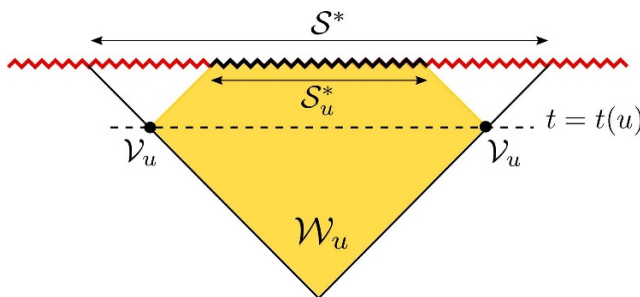
Figure 14. WdW patch for a Kasner slab \mathcal{S}_u^* = [-\frac{u}{2}, \frac{u}{2}] \times \mathbf{R}^{d-1} .
