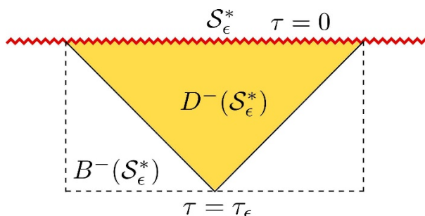
Figure 9. Comparison between the \epsilon -box and the past domain of dependence of \mathcal{S}_\epsilon^* .
