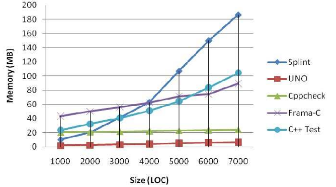
Figure 5. Average of peak memory usage in three cases: path-sensitive, context-sensitive and alias analysis
