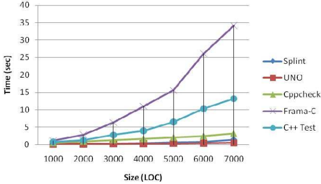
Figure 4. Average time for three analysis cases: path-sensitive, context-sensitive and alias analysis
