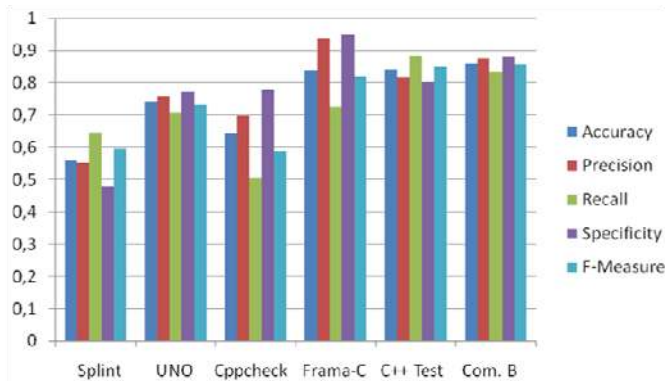
Figure 2. Tool effectiveness on the considered C code defects
