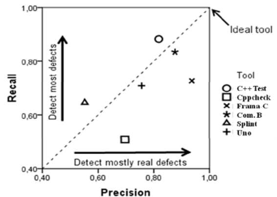
Figure 3. How the tools balance the tradeoff between precision and recall
