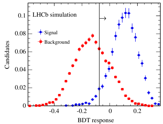
FIG. 11. Distribution of the BDT response on the signal and background simulated samples.
