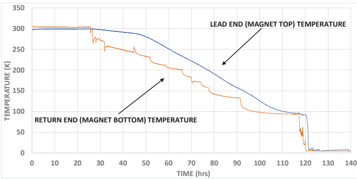
Fig. 2. Temperature plot of MQXFA04 second cooldown.
