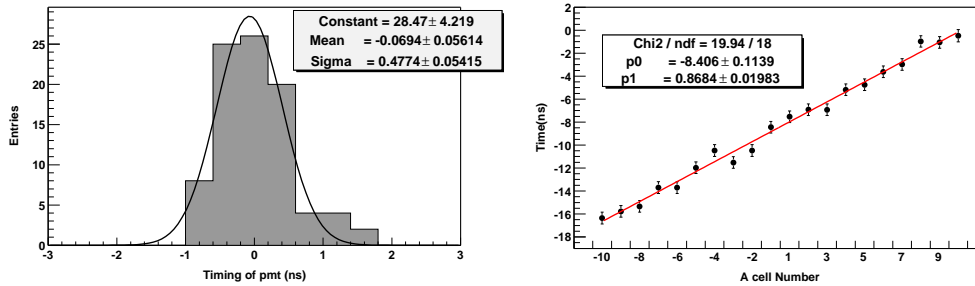
Fig. A.3. On the left, the difference in time between the generic channel and the reference one once the corrections for the delays introduced by the clear fibers inside the module have been taken into account. On the right, the timing of a muon impinging at 90^\circ on the A cells. The slope indicates a value of 31 \pm 2 cm/ns for the speed of the muon.
