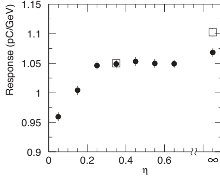
Fig. 22. The dependence of the EM calibration constants on the pseudorapidity. The results of the simulation for 20 GeV electrons is shown by full circles. Open squares represent two experimental points, for \eta = 0.35 ( \theta_{\text{TB}} = 20^\circ ) and \eta = \infty ( \theta_{\text{TB}} = 90^\circ ). The simulated data are normalized to the experimental data at \eta = 0.35 .
