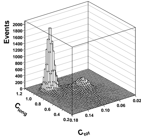
Fig. 15. The combination of the quantities C_{\text{long}} and C_{\text{tot}} used for electron/hadron separation at 180 GeV. The region on the left corresponds to electrons, the other to hadrons.
