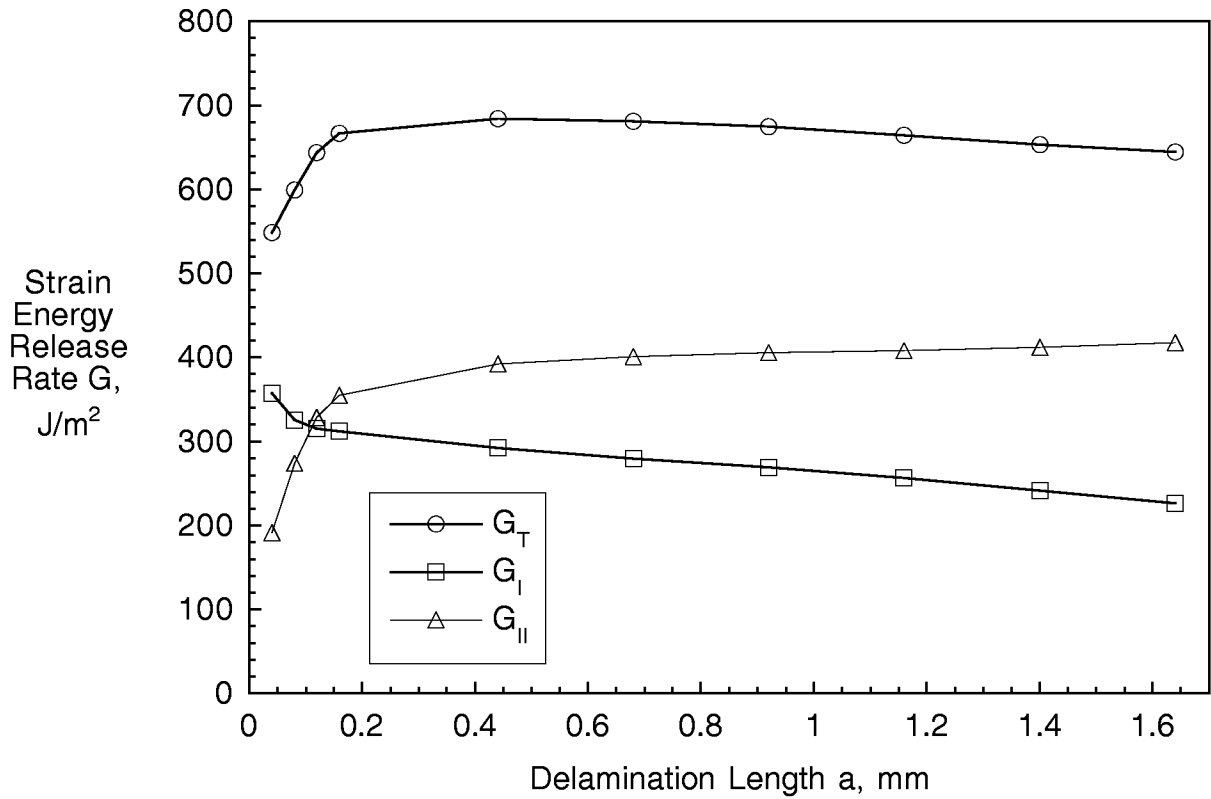
Figure 37. Computed Strain Energy Release Rates for Delamination Growth Between Adhesive and 0^\circ Skin Ply for ATB Tests.
