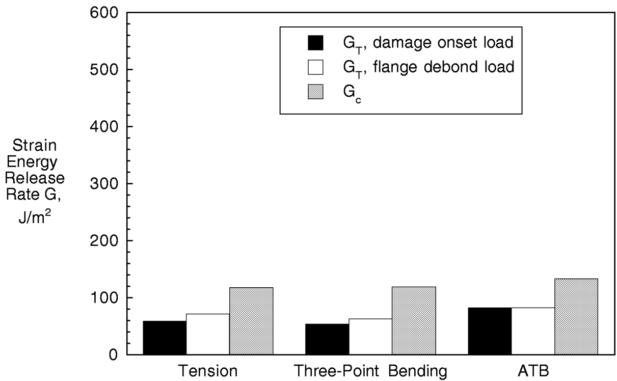
Figure 45. Comparison of Computed Total Strain Energy Release Rates in a 90°/45° Flange Ply Interface with Mixed-Mode Fracture Toughnesses.
