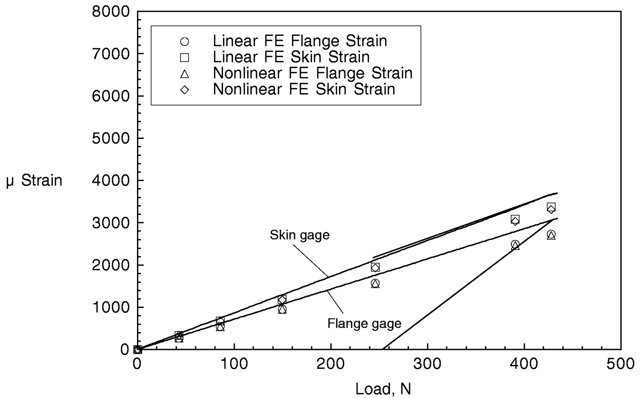
Figure 24. Comparison of Measured Strains with Computed Results for Three-Point Bending Load Case.
