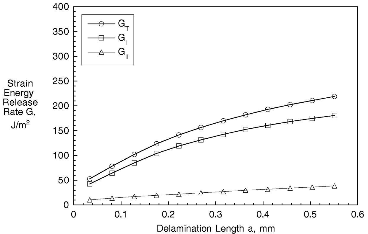
Figure 32. Computed Strain Energy Release Rates for Delamination Growth in a 90^\circ/45^\circ Flange Ply Interface for Three-Point Bending Tests.
