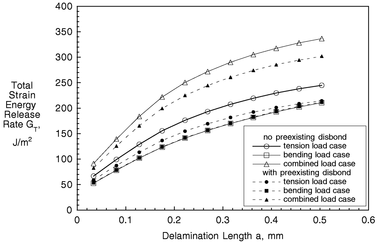
Figure 44. Computed Strain Energy Release Rates for Delamination Growth in a 90°/45° Flange Ply Interface with and without a Preexisting Disbond Between Adhesive and 0° Skin Ply.
