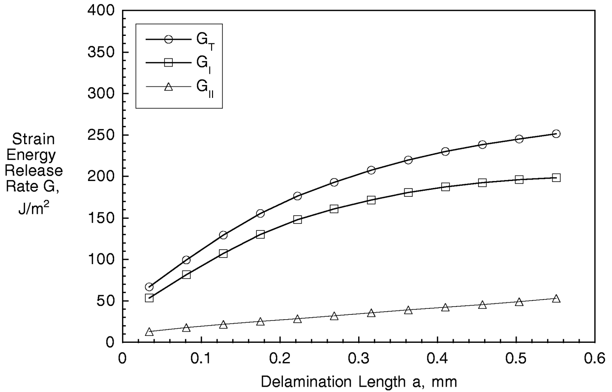
Figure 31. Computed Strain Energy Release Rates for Delamination Growth in a 90^\circ/45^\circ Flange Ply Interface for Tension Tests.
