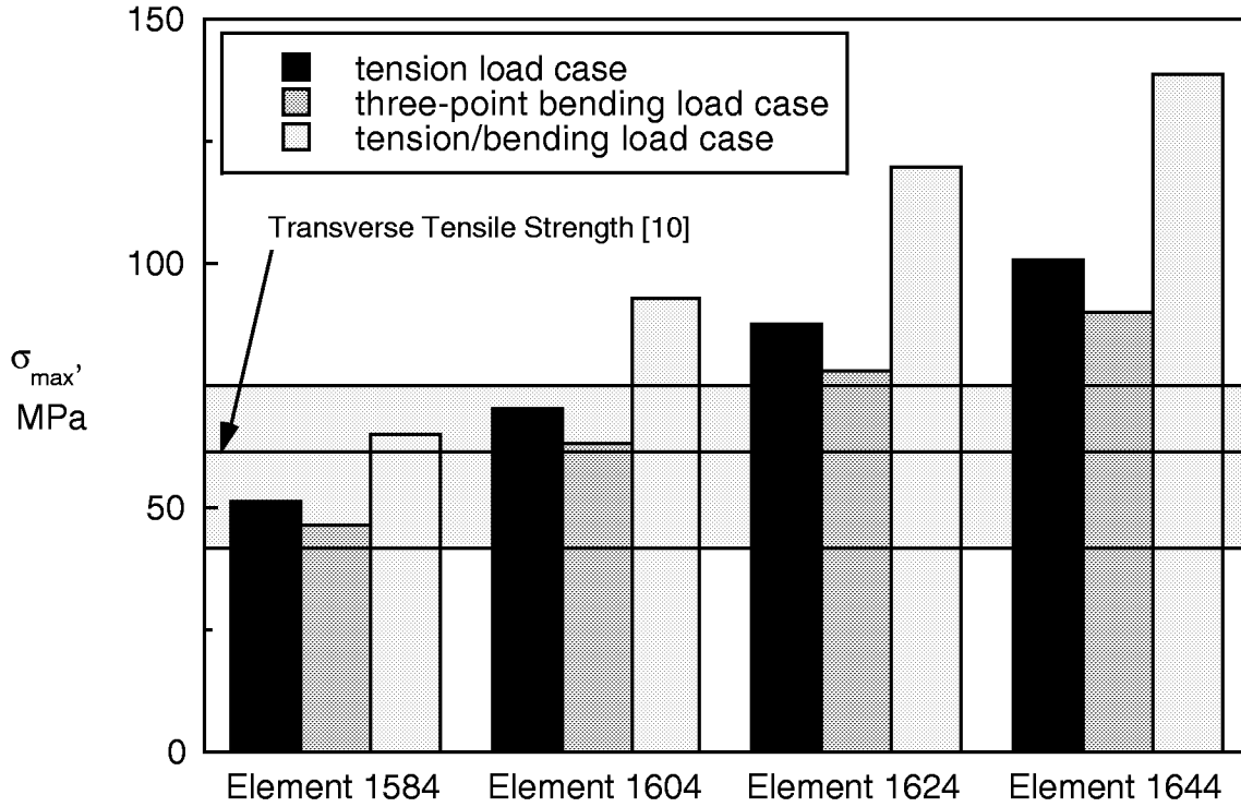
Figure 30. Comparison of Principal Tensile Stresses Computed at Damage Initiation Load.
