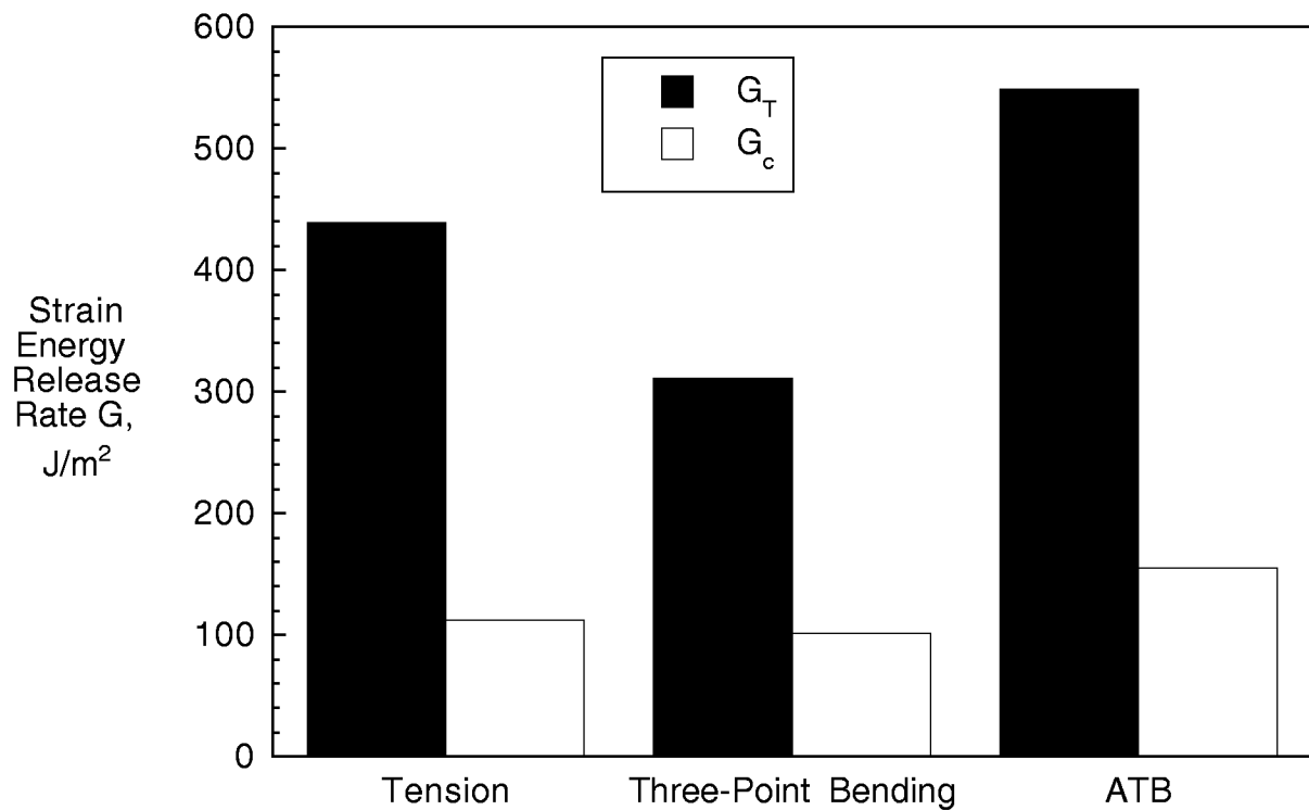
Figure 41. Comparison of Computed Total Strain Energy Release Rates in a 0° Skin Ply/Adhesive Film Interface with Mixed-Mode Fracture Toughnesses.
