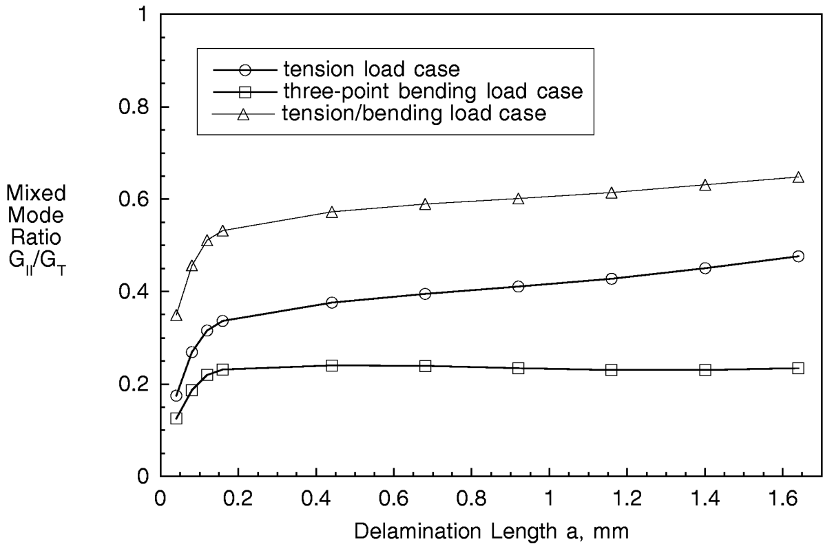
Figure 38. Computed Mixed Mode Ratios for Delamination Growth Between Adhesive and 0^\circ Skin Ply.
