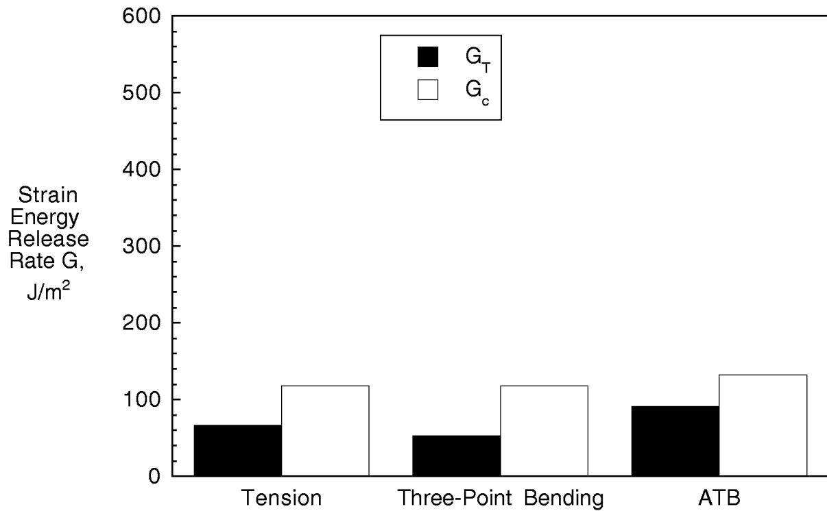
Figure 40. Comparison of Computed Total Strain Energy Release Rates in a 90°/45° Flange Ply Interface with Mixed-Mode Fracture Toughnesses.
