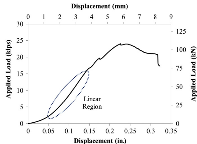
Fig. 12. Average load–displacement curve for crushing test
