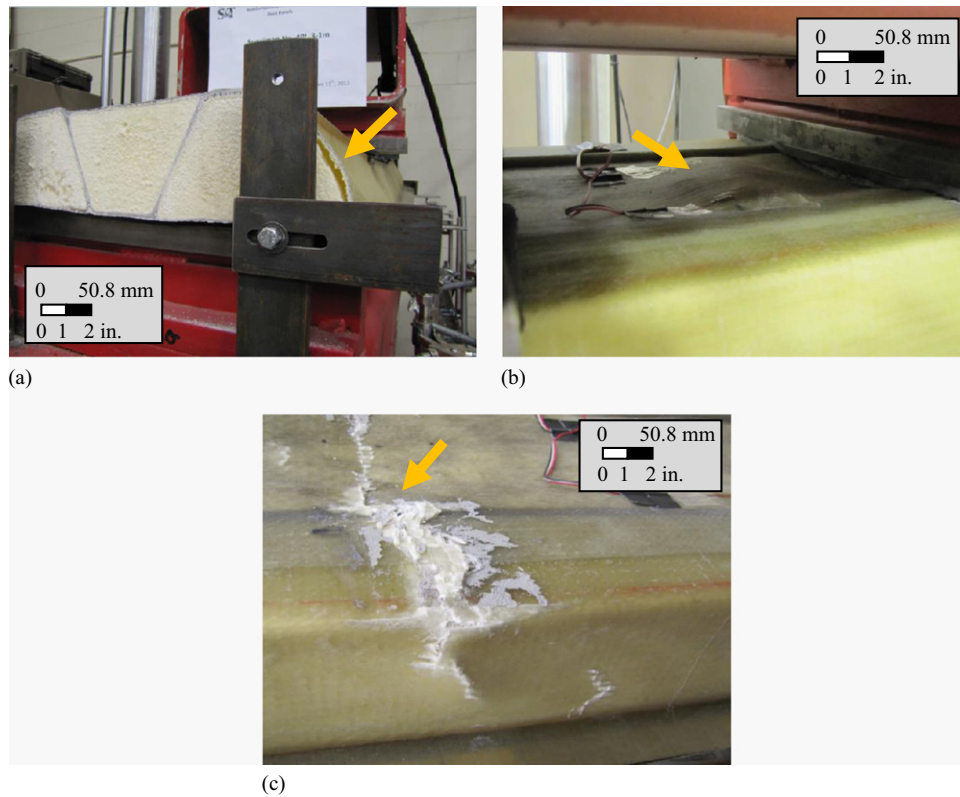
Fig. 21. Failure modes: (a) delamination; (b) outward facing wrinkling; and (c) compression failure
