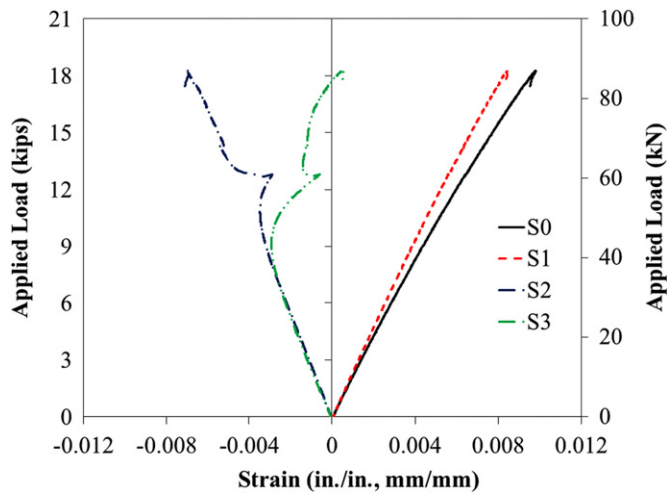
Fig. 17. Load-strain curves for the top and bottom facings
