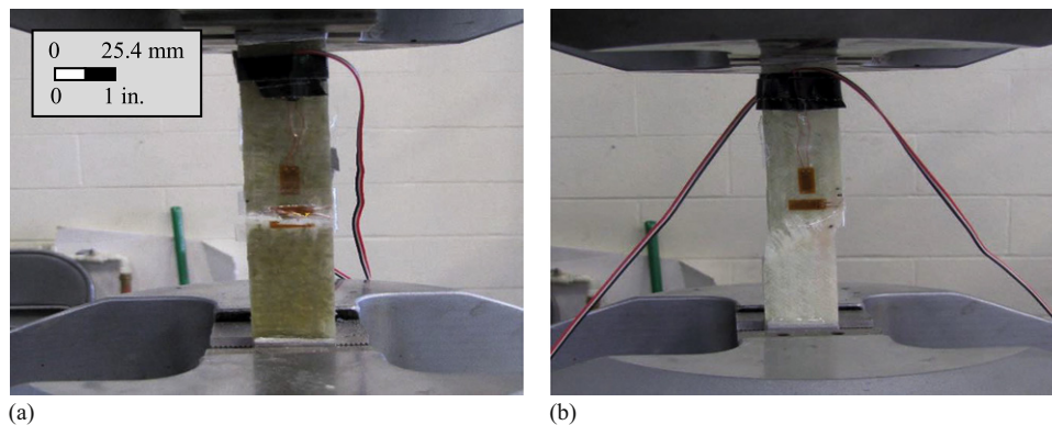
Fig. 3. Failure of (a) GFRP facings; (b) web layers
