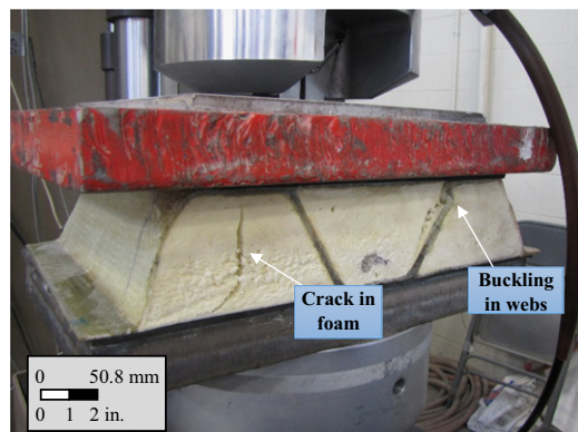
Fig. 13. Failure of specimen subject to crushing test
