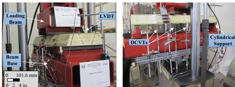
Fig. 8. Four-point bending test setup for the flexure test
