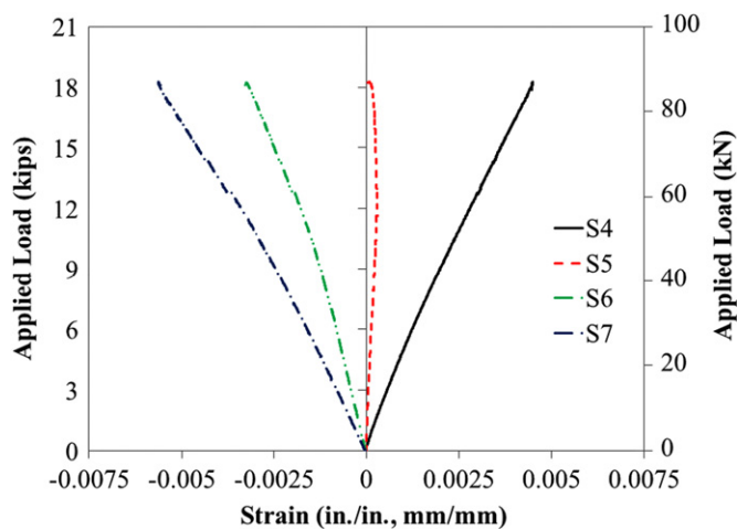
Fig. 18. Load-strain behavior of sandwich panel
