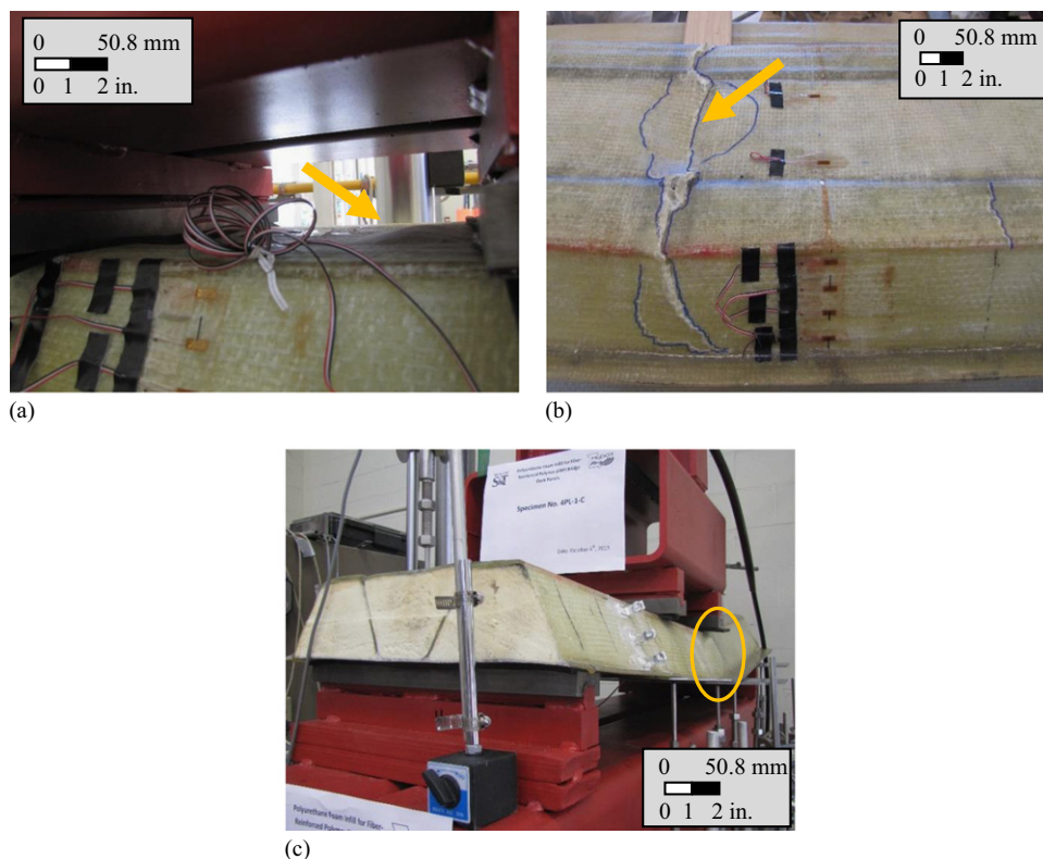
Fig. 16. Failure modes: (a) initial failure due to outward compression facing wrinkling; (b) ultimate failure due to compression failure of the facing under loading point; and (c) final failure mode triggered by crushing
