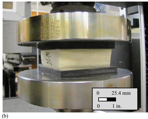
Fig. 6. Flatwise compressive test: (a) average compressive stress–strain curves; (b) test setup
