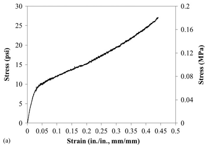
Fig. 6. Flatwise compressive test: (a) average compressive stress–strain curves; (b) test setup
