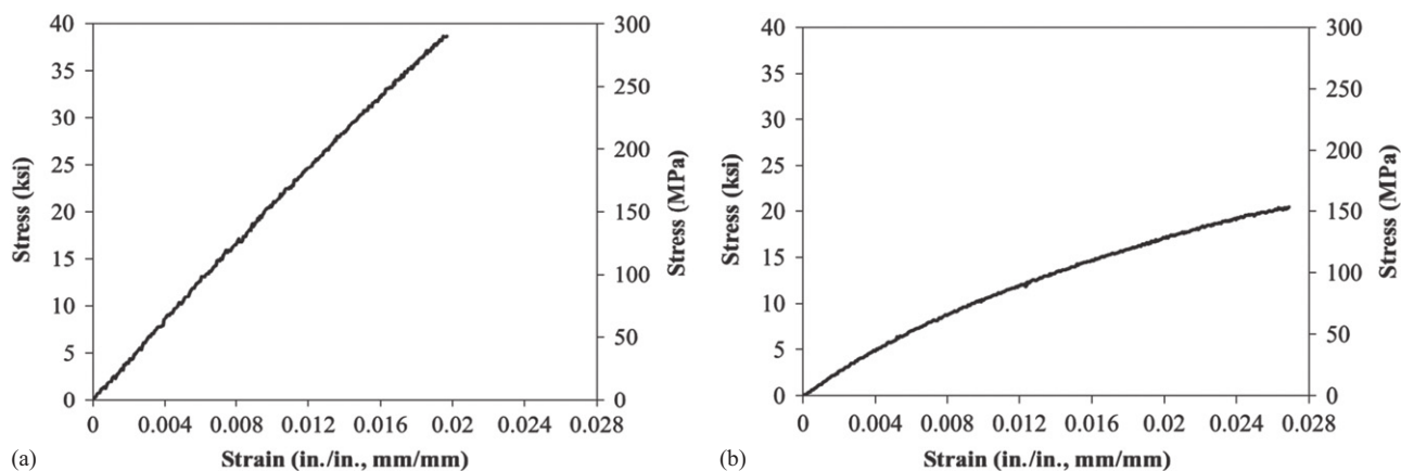
Fig. 4. Average tensile stress–strain curves for (a) GFRP facings; (b) web layers
