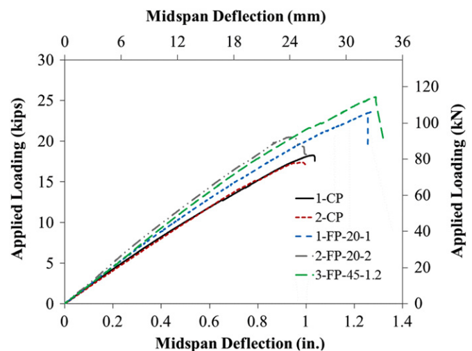
Fig. 20. Load versus midspan deflection for control and fatigued panels
