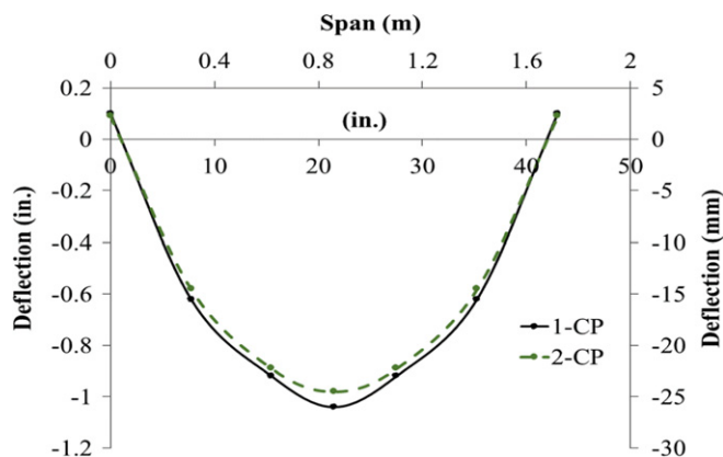
Fig. 15. Deflection profile along span length during flexure test
