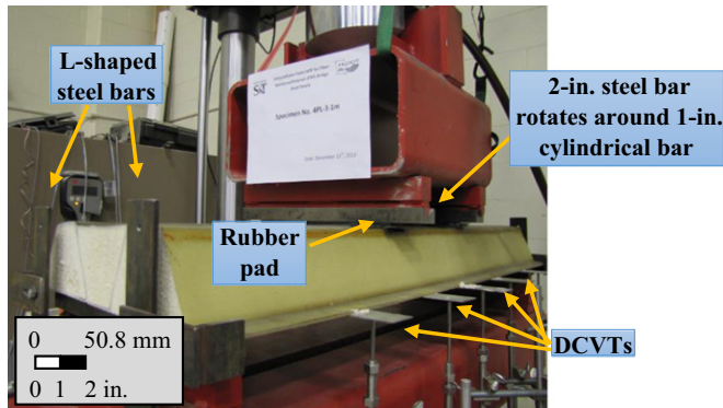
Fig. 11. Four-point bending test setup for the fatigue test
