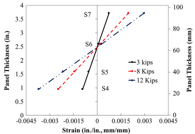
Fig. 19. Strain distribution through the thickness for strain gauges S4, S5, S6, and S7
