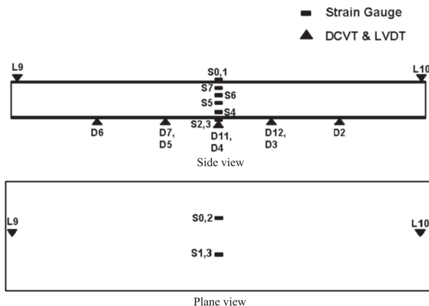
Fig. 10. Schematic of instrumentation locations
