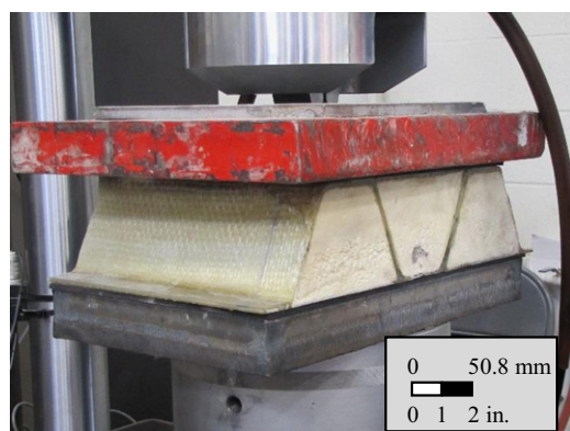
Fig. 7. Crushing test setup
