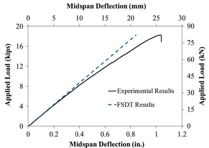
Fig. 23. Comparison between experimental results and theoretical predictions by the FSDT theory
