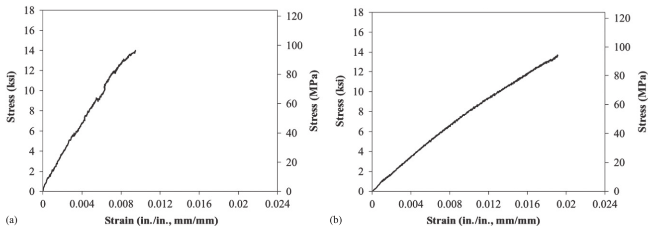
Fig. 5. Average compressive stress–strain curves for (a) GFRP facings; (b) web layers
