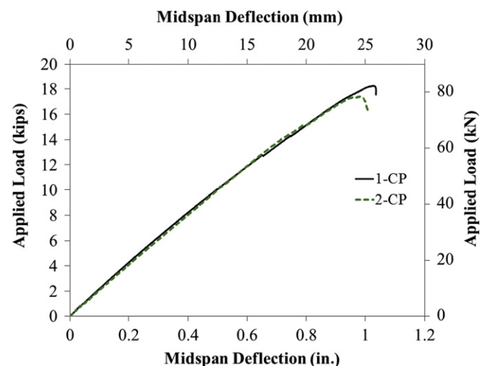
Fig. 14. Load versus midspan deflection for flexure test
