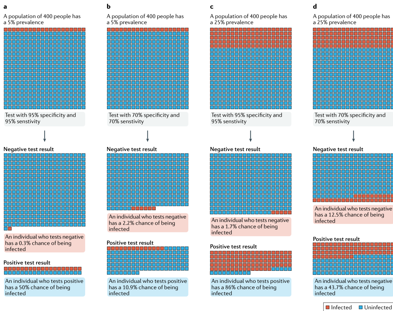
Fig. 2 | How test sensitivity, specificity and disease prevalence influence the interpretation of test results. a,b | In a population with a low prevalence (5% here) of COVID-19 cases, even a highly sensitive and specific test (part a ) returns many false-positive results. c,d | By contrast, a high infection prevalence (25% here) increases the likelihood that a positive result is true, despite the test performance remaining unchanged. The positive predictive value (PPV) of a test describes the probability that an individual who tests positive is actually infected 35 , and thus depends on both the specificity of the test and the prevalence of infection. At low prevalence values, the proportion of false-positive results is increased and the PPV is reduced. Even a highly specific test returns mostly false-positive results (and therefore has a low PPV) when the prevalence of infection is low. Adapted from REF. 134 , Springer Nature Limited.
