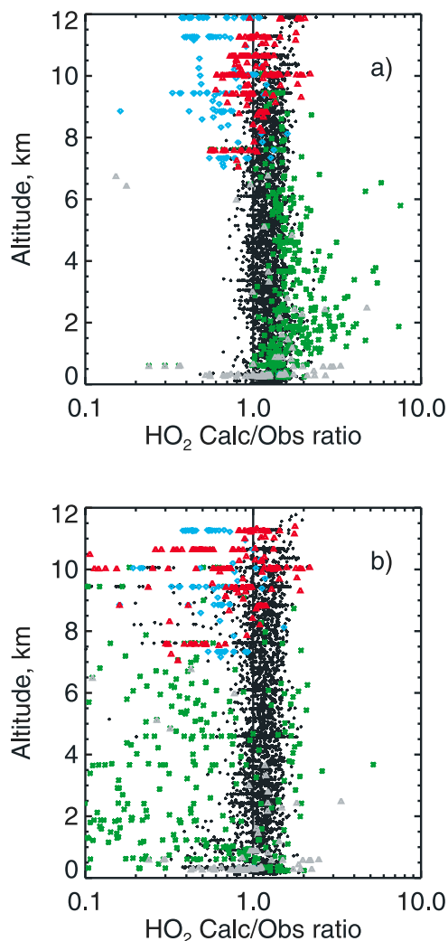
Figure 5. Subsets for HO 2 calc/obs ratios on the DC-8. (a) HO 2 calc/obs ratio versus altitude for the DC-8 aircraft. Blue diamonds indicate data with O_3 > 120 ppbv (stratospheric data). Red triangles indicate data with NO > 135 pptv for altitudes above 7 km, and gray triangles indicate high NO data for altitudes below 7 km. Green asterisks show data points that were identified as residing in clouds, using criteria described in the text. (b) Results from a test simulation including a heterogeneous loss of HO 2 to clouds and aerosols, so only data points containing the FSSP measurements described in the text (necessary to calculate the heterogeneous loss rate) are shown. Subsets are identified as in Figure 5a.
