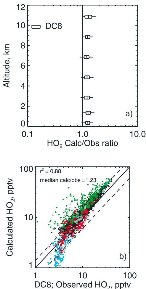
Figure 4. Comparison of calculated and observed HO 2 from the DC-8 aircraft. (a) Calculations of HO 2 relative to observed values for the DC-8 aircraft. See Figure 1 caption for definition of box and whiskers. (b) A scatterplot of observed HO 2 versus calculated HO 2 for the DC-8 aircraft. Measurement uncertainties of \pm 40\% are indicated by the dashed lines in Figure 4b. Subsets for the HO 2 calculated-to-observed ratios discussed in the text are also indicated in Figure 4b. Blue diamonds indicate data with O_3 > 120 ppbv (stratospheric subset). Red triangles indicate data with NO > 135 pptv for altitudes above 7 km, and gray triangles indicate high NO data for altitudes below 7 km. Green asterisks show data points that were identified as residing in clouds, using the criteria described in the text.
