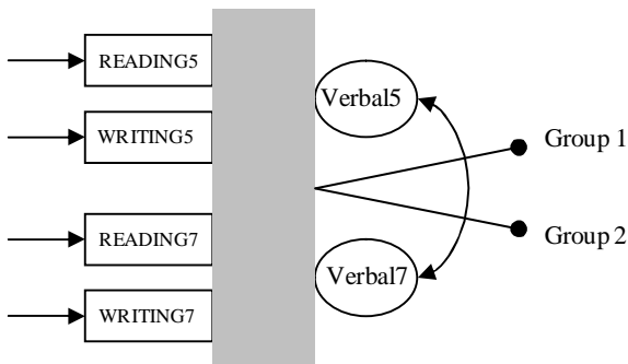
Figure 2c. Scalar invariance (same item intercepts across groups)
