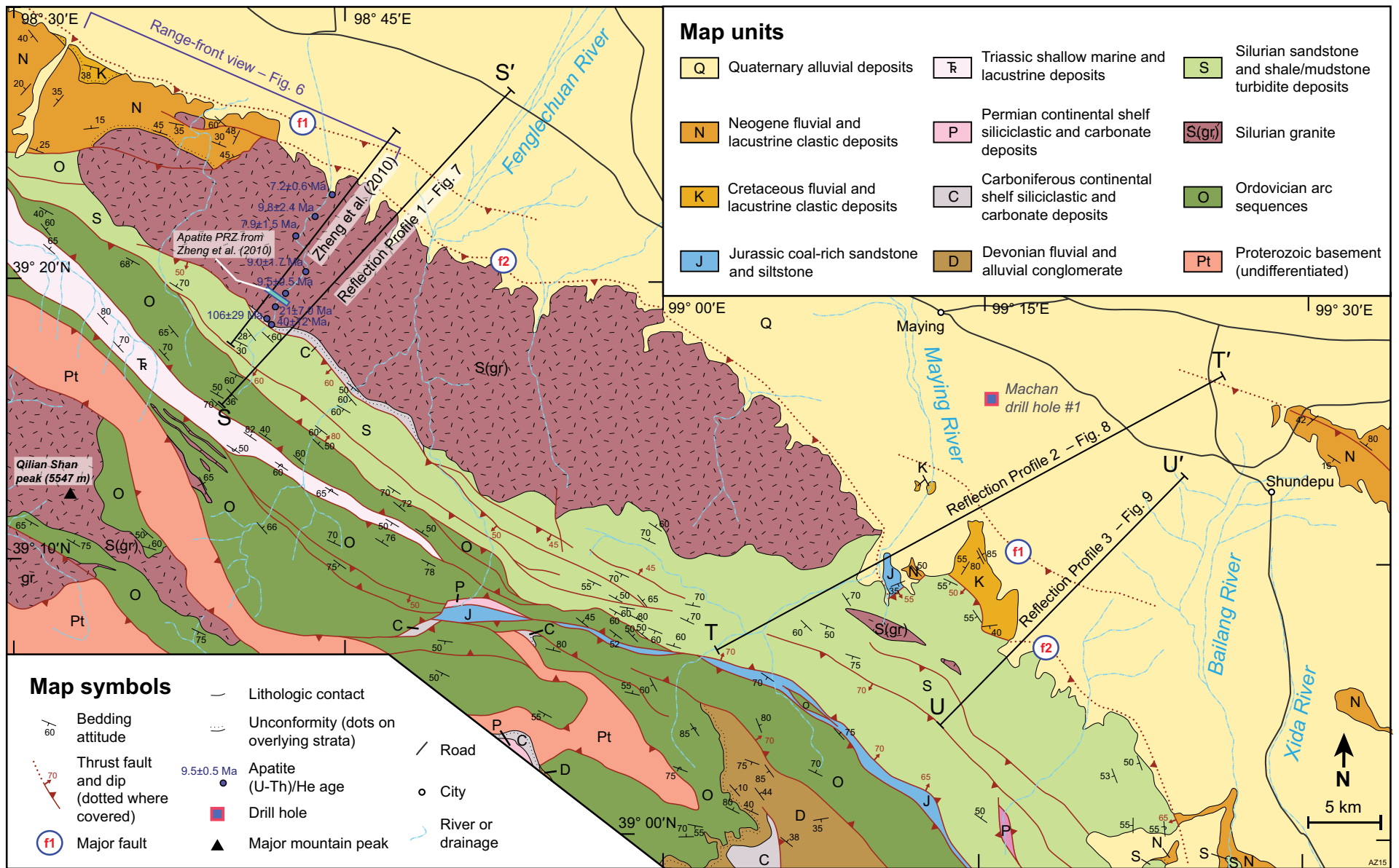
Figure 5. Geologic map across the northern Qilian Shan frontal thrust zone compiled from unpublished maps, Gansu Geological Bureau (1989), Qinghai BGMR (1991), and our own structural interpretations. See Figure 1 for location. Satellite image viewpoint (Google Earth) of Figure 6 is shown. Also shown are the locations of three seismic reflection profiles (Figs. 7–9), a drill hole described in J. Wu et al. (2006), and the AHe traverse of Zheng et al. (2010). PRZ—partial retention zone.
