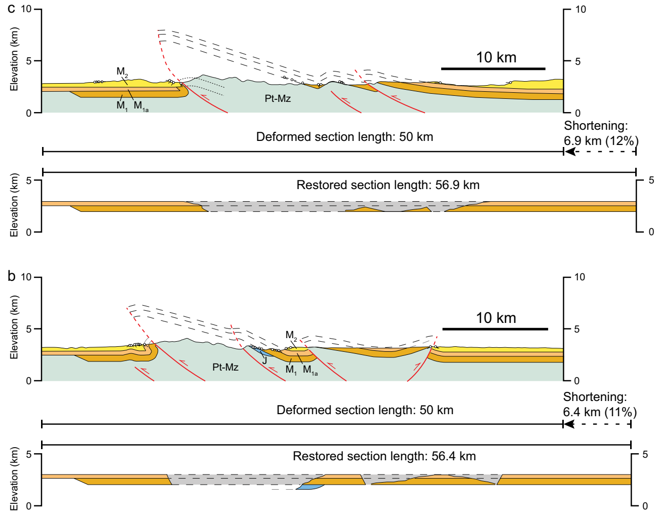
Figure 4 (continued). (E) Two of three north-south cross sections across the Gonghe Nan Shan by Craddock et al. (2014). These sections assume that the tilted Cenozoic strata are forelimbs and backlimbs of fault-bend folds. Deformation within pre-Miocene units is not considered. Ar—Archean; C—Carboniferous; E—Eocene; J—Jurassic; K—Cretaceous; Mz—Mesozoic; N—Neogene; O(gr)—Ordovician granite; P—Paleogene; Pt—Proterozoic; Pz—Paleozoic; Q—Quaternary; S—Silurian; Tr—Triassic; Vp—P wave velocity.
