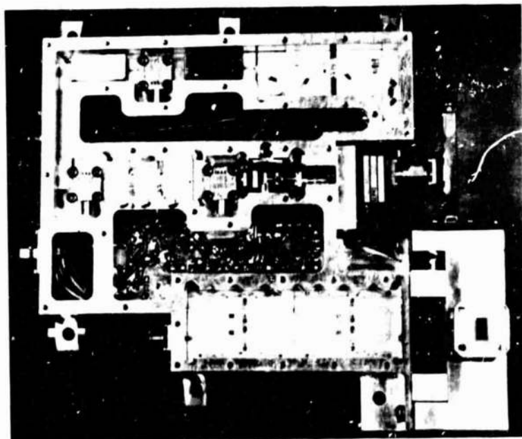
Figure 2. MT receiver.
