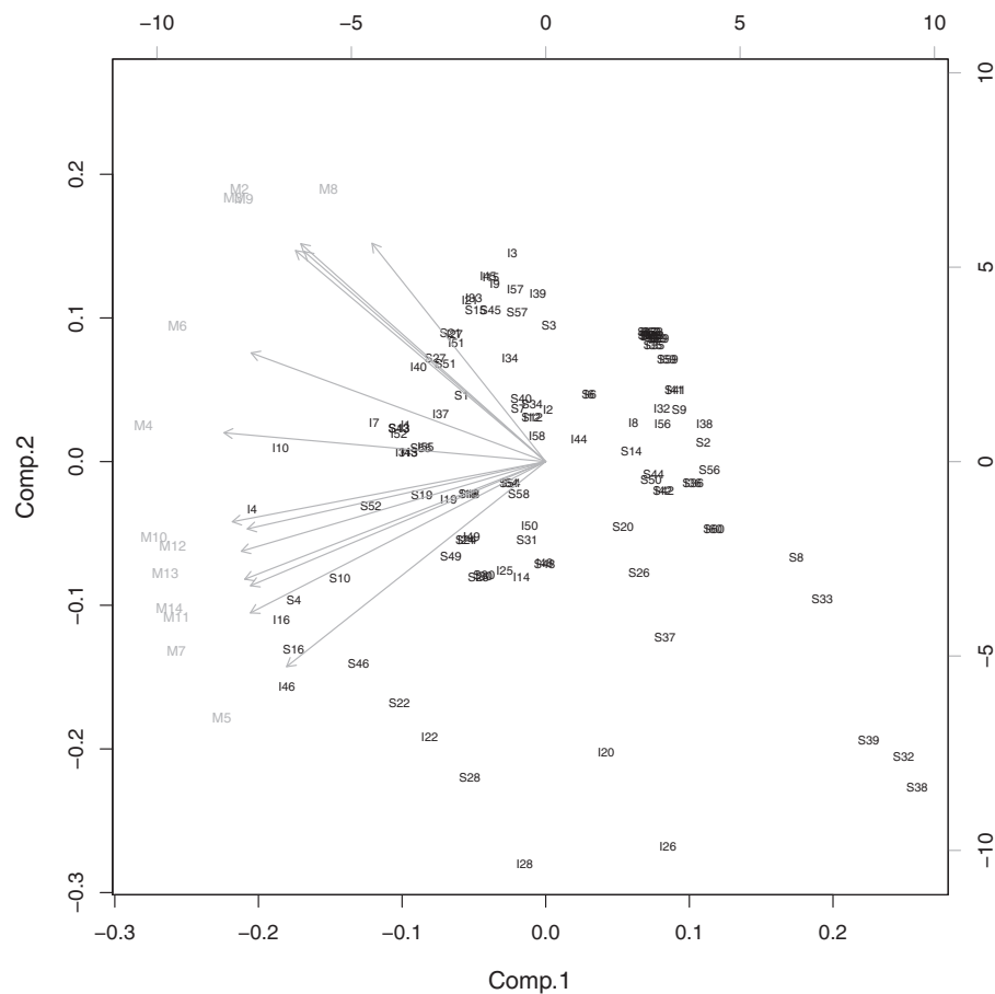
Fig. 1: Biplot for the simulations related to the Gaussian noise.
