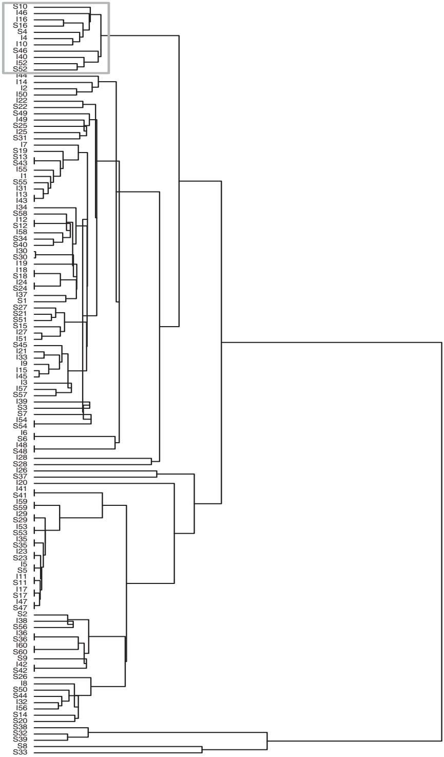
Fig. 2: Dendrogram for the simulations related to the Gaussian noise.
