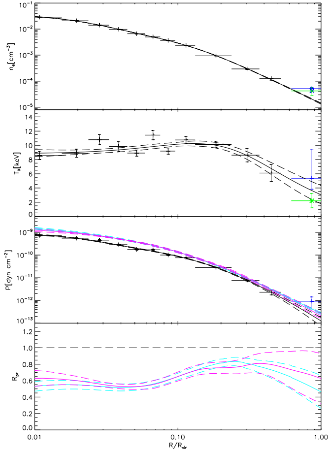
Figure 3. Top three panels: radial profiles of electron density and temperature, and thermal pressure in A1689 derived from Chandra observations (black points with error bars), and adopted from Suzaku observations (blue points with error bars; offset 1; Kawaharada et al. 2010). In the top two panels, we also show the best-fit models (black solid lines), and, as a reference, the last point of offset 2 of Suzaku (green stars with error bars). In the third panel, the black solid line is derived from the density and temperature fits. In this panel, we also show hydrostatic equilibrium pressure, P_{\text{he}} , derived from gravitational lensing using an NFW and a non-parametric model for the total mass distribution (cyan and magenta solid lines). Pressure ratios, R_{\text{pr}} = P_{\text{th}}/P_{\text{he}} , are shown in the bottom panel (color code is the same as in the third panel; horizontal black dashed line represents ratio of unity).
