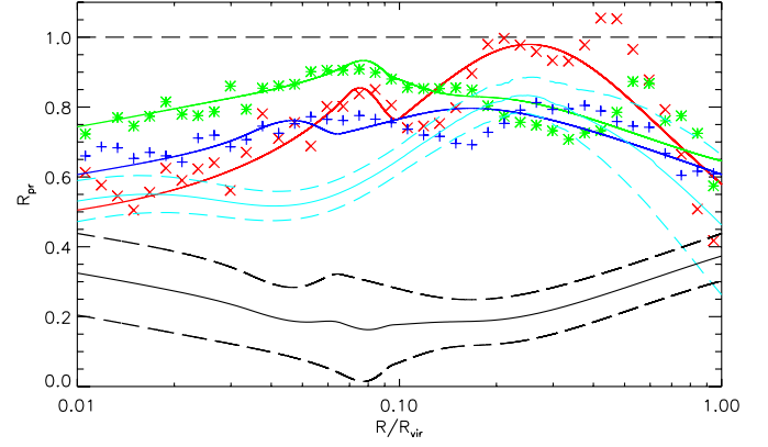
Figure 2. Pressure ratio profiles, P_{\text{th}}/P_{\text{he}} derived for simulated massive clusters CL1, CL2, and CL3 (code is the same for the colored solid lines and points (as in Figure 1), and for A1689 using the latest NFW lensing model (cyan lines, same as in Figure 3)). We also show the average dynamical pressure ratios, (P_{\text{dyn}}/P_{\text{he}}) , for simulated relaxed clusters CL1 and CL2 with errors (black lines). See the text for details and the definition of errors (dashed lines).
