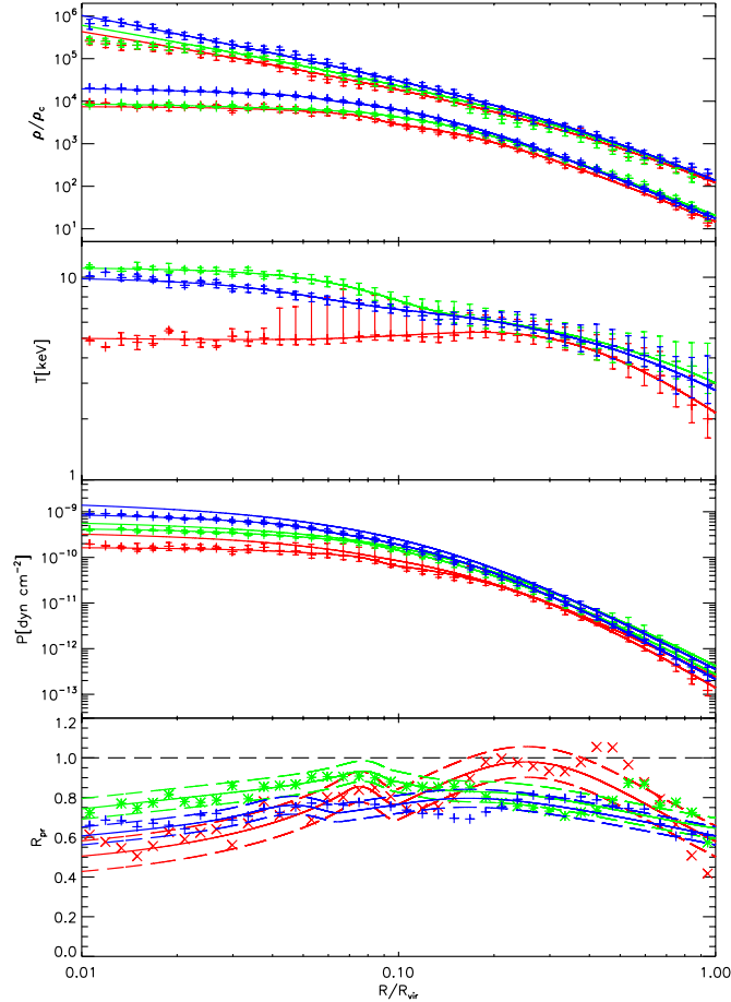
Figure 1. From top to bottom: radial profiles of dark matter and gas density (upper and lower curves) in units of critical density, \rho_c ; gas temperature (in keV); hydrostatic and thermal gas pressure (upper and lower curves, in \text{dyn cm}^{-2} ); and pressure ratios, P_{\text{th}}/P_{\text{he}} , for massive simulated clusters. Solid lines and points with error bars represent best-fit models and data points for our relaxed clusters (blue: CL1; green: CL2), and for a cluster with a non-relaxed core (red: CL3). We also show pressure ratios using gas pressure data points (blue plus signs, green stars, and red crosses; see the text for details).
