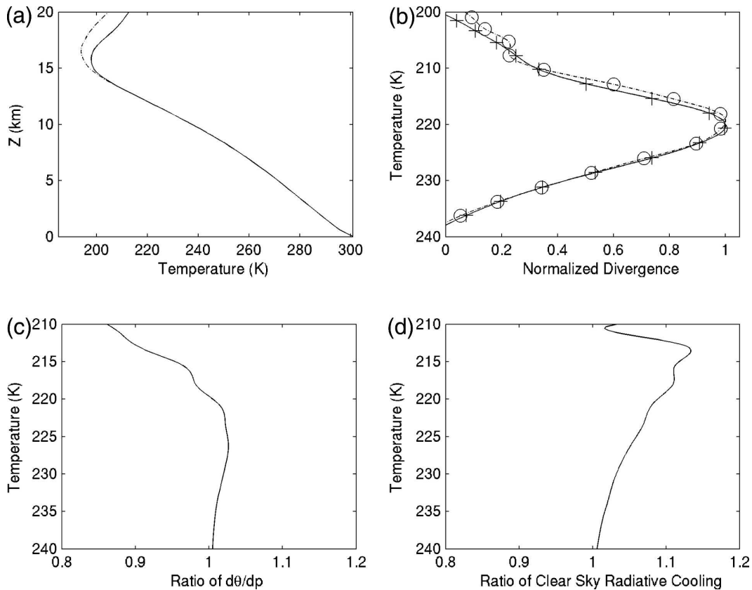
FIG. 5. The (a) temperature profile and (b) normalized divergence as functions of temperature for the control case (solid, +) and the case with dynamical cooling in the stratosphere (dashed-dotted, circle). The ratio of (c) d\theta/dp and (d) clear-sky radiative cooling of the dynamical cooling case to the control case.
