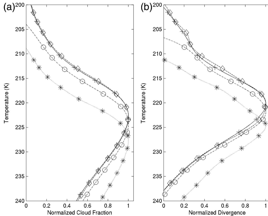
FIG. 3. Normalized (a) cloud fraction and (b) divergence as functions of temperature with the ozone profile shifted by +8 km (diamond), 0 km (+), -4 km (circle), and -12 km (*). The SST is 30.5°C.
