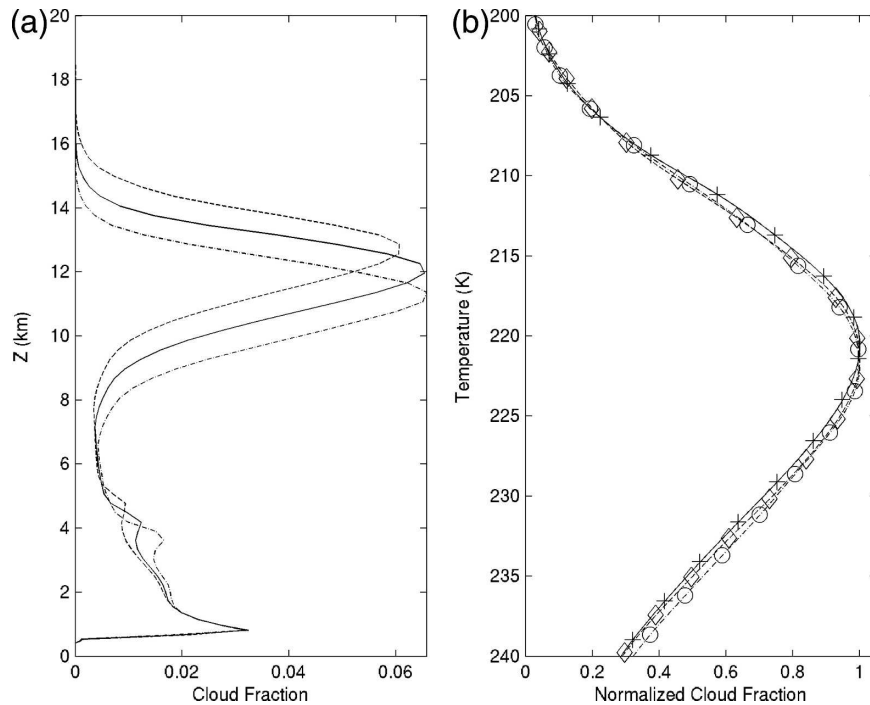
FIG. 6. RCE profiles of cloud fraction as a function of (a) height and (b) temperature for SSTs of 32.5° (dashed, diamond), 30.5° (solid, +), and 28.5°C (dashed-dotted, circle) using the Krueger microphysics.
