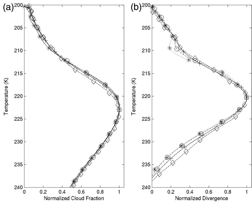
FIG. 2. Normalized (a) cloud fraction and (b) divergence estimated from Eq. (1) as functions of temperature for SSTs of 32.5° (dashed, diamond), 30.5° (solid, +), 28.5° (dashed-dotted, circle), and 26.5°C (dotted, *).
