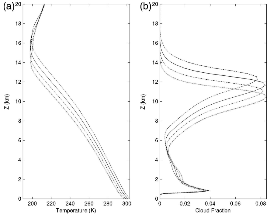
FIG. 1. RCE profiles of (a) temperature and (b) cloud fraction for SSTs of 32.5° (dashed), 30.5° (solid), 28.5° (dashed-dotted), and 26.5°C (dotted).
