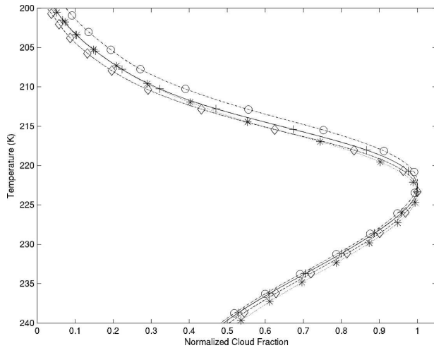
FIG. 4. Normalized cloud fractions as a function of temperature for the control case (solid, +) and cases with doubled CO 2 (dotted, *), doubled stratospheric water (dashed, diamond), and dynamical cooling in the stratosphere (dashed-dotted, circle).
