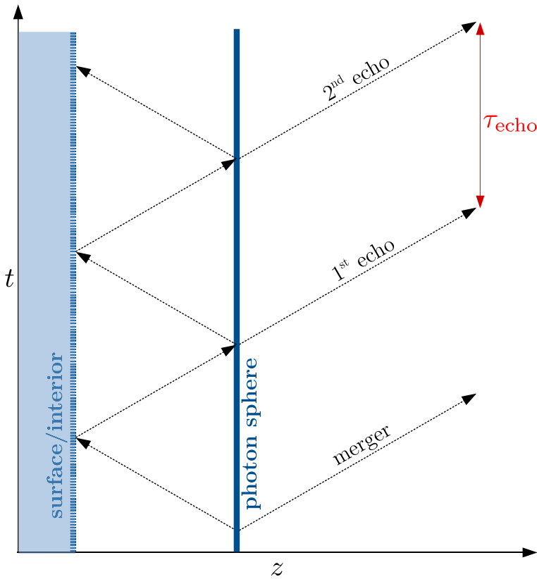
Fig. 10 Schematic Penrose diagram of GW echoes from an ECO. Adapted from Abedi et al. (2017a) [similar versions of this plot appeared in other contexts in Vilenkin (1978) and Mark et al. (2017)]
