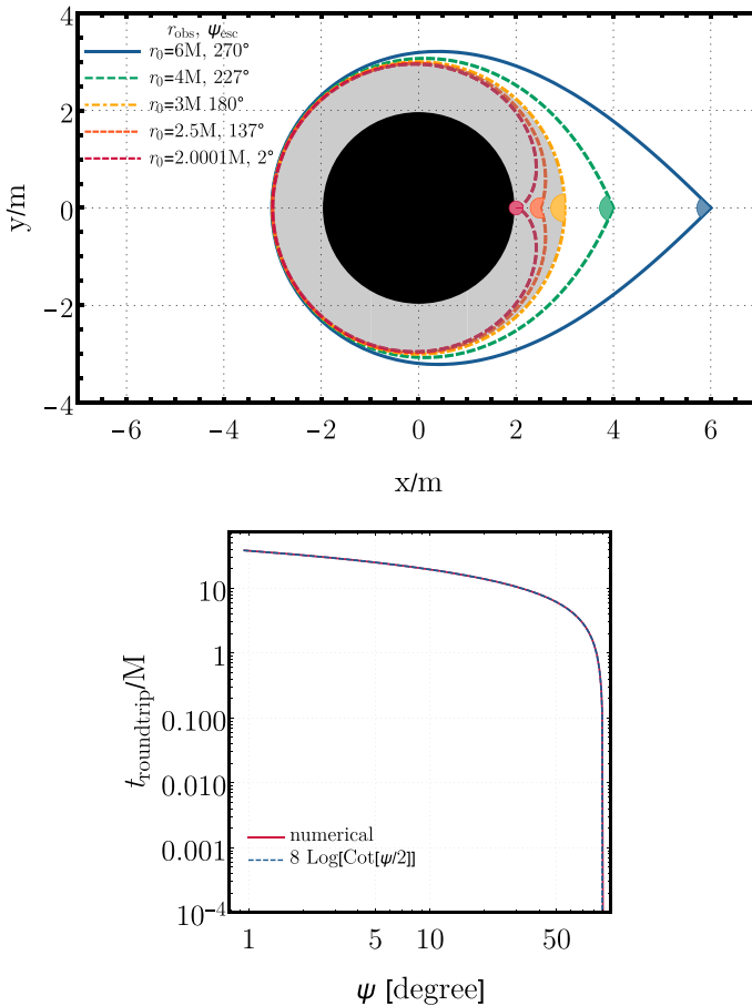
Fig. 3 Top: Critical escape trajectories of radiation in the Schwarzschild geometry. A locally static observer (located at r = r_{\text{obs}} ) emits photons isotropically, but those emitted within the colored conical sectors will not reach infinity. The gray shaded area is the photon sphere. Bottom: Coordinate roundtrip time of photons as a function of the emission angle \psi > \psi_{\text{esc}} and for \epsilon \ll 1
