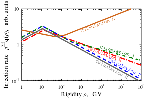
Figure 1: Galactic CR source injection spectrum in Calculations R, P, I, L and H . Units are arbitrary. The normalisation of the injection spectrum was chosen to obtain the best fit of proton and He spectrum at Earth. For all calculations, the lines represent the Galactic CR source injection spectrum. The local sources, present in Calculation L and Calculation H , are not shown here. The local source fluxes at Earth in Calculation L and Calculation H were obtained as the difference between the observed and the propagated Galactic fluxes.
