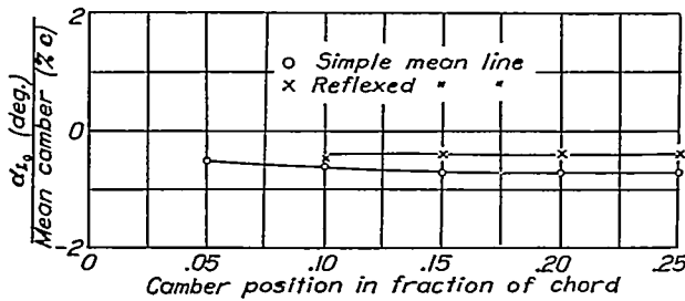
FIGURE 12.—Variation of angle of zero lift with camber position.
