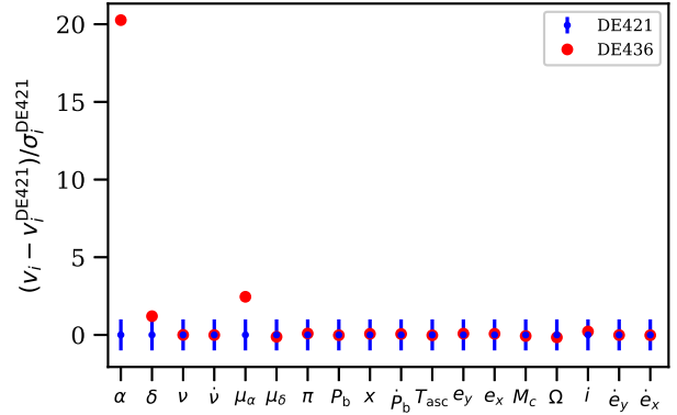
Figure 1. A comparison between DE436 and DE421 timing solution when fitting a simulated dataset. The plot shows (v_i - v_i^{\text{DE421}}) / \sigma_i^{\text{DE421}} , where v_i is the value of parameter i and \sigma_i is the uncertainty of parameter i from Table 1. The blue error bars indicate the DE421-based timing parameters with their uncertainties scaled to unity, while the red dots are the DE436-based parameters we get from fitting the simulated dataset.
