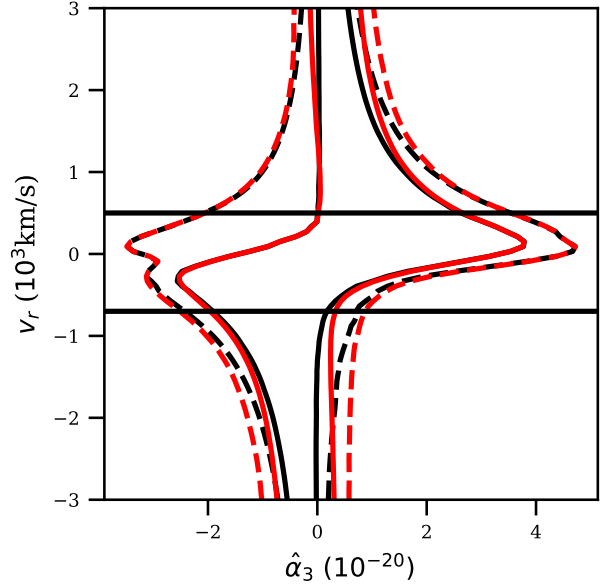
Figure 4. The likelihood distribution of \hat{\alpha}_3 derived from the MCMC of PSR J1713+0747's timing and noise parameters as a function of the assumed line-of-sight velocity v_r . The black solid curves corresponds to the 95% C.L. and the black dashed line to the 99% C.L. The red curves shows the same limits with \hat{\alpha}_1 taken into account (see Section 2.4 for details). The two horizontal lines labels the escape velocity of the pulsar binary.
