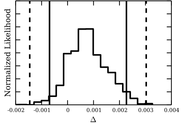
Figure 3. The normalized likelihood distribution of \Delta derived from the MCMC of PSR J1713+0747’s timing and noise parameters. Solid line is the 95% confidence limit, dashed line marks the 99% confidence limit.
