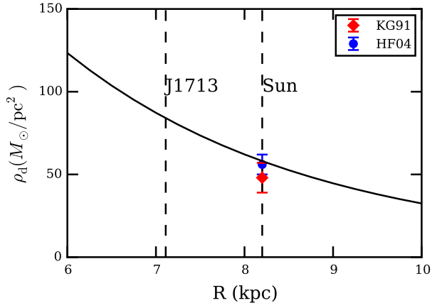
Figure A1. The solid curves show the models of Galactic disk surface density as a function of Galactic radius from McMillan (2017) . The error bars indicate disk surface densities from studies of the dynamics of stars in the Solar vicinity by Kuijken & Gilmore (1991) (red diamond) and Holmberg & Flynn (2004) (blue circle). The vertical lines mark the positions of the pulsar and the Sun.
