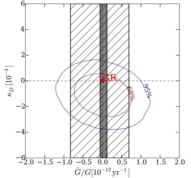
Figure 2. Confidence contours of \dot{G}/G and \kappa_D computed from MCMC simulations based on timing results of PSRs J0437–4715, J1738+0333, and J1713+0747. The shaded area and gray area mark the 95% confidence limit from LLR ( Hofmann et al. 2010 ) and planetary ephemerides ( Fienga et al. 2015 ), respectively.
