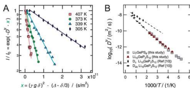
Fig. 2 ^7\text{Li} PFG NMR on \text{Li}_7\text{GePS}_8 and \text{Li}_{10}\text{GeP}_2\text{S}_{12} . (A): echo attenuation curves for selected temperatures ( \text{Li}_7\text{GePS}_8 ). (B): tracer diffusion coefficients extracted from the echo attenuation. At all temperatures, the diffusion time \Delta was set short enough to avoid finite crystallite size effects (cf. ESI†).
