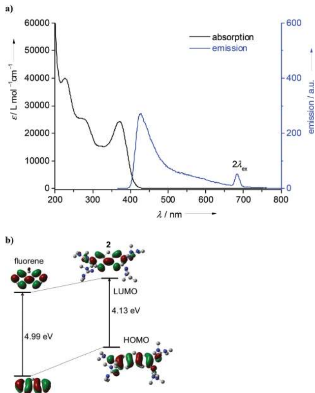
Fig. 5 (a) Electronic absorption and emission spectra for 2 in CH 3 CN solution. (b) Calculated HOMO and LUMO energies (B3LYP/6-311G**) of 2 relative to unsubstituted fluorene.
