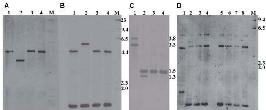
Fig. 4. RFLP of mtDNA from diploid lines hybridized with mitochondrial probes. DNA digested with Eco RI and probed with m79 (A), m93 (B) and m112 (D). DNA digested with Hind III and probed with m112 (C). Lanes: 1-2B, 2-3C, 3-4D, 4-5E, 5-13M, 6-14N, 7-15O, 8-16P.
