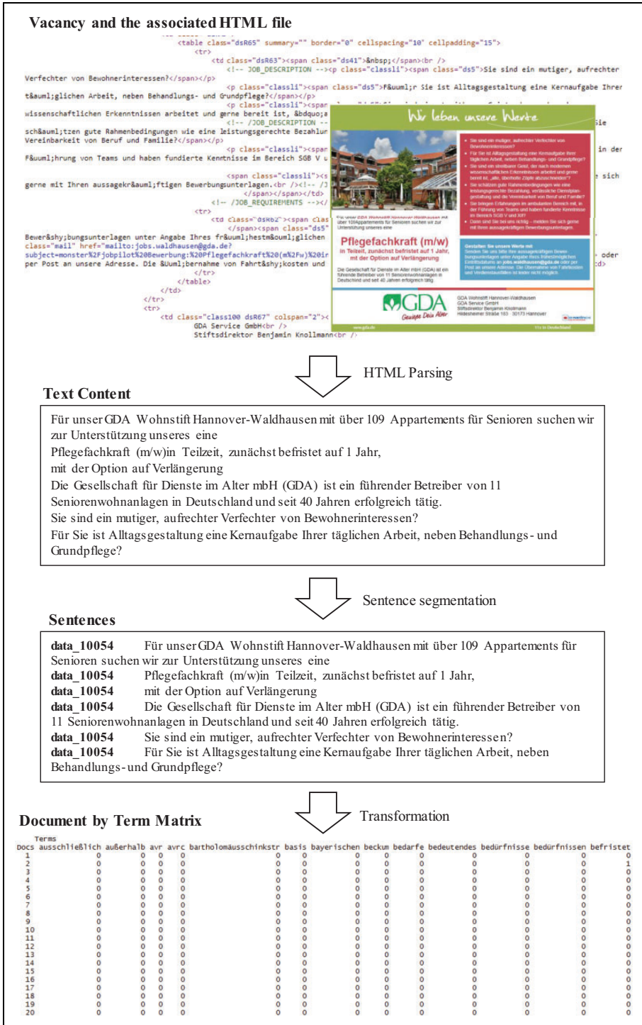
Figure 3. Illustration of text preprocessing from raw HTML file to document-by-term matrix.
