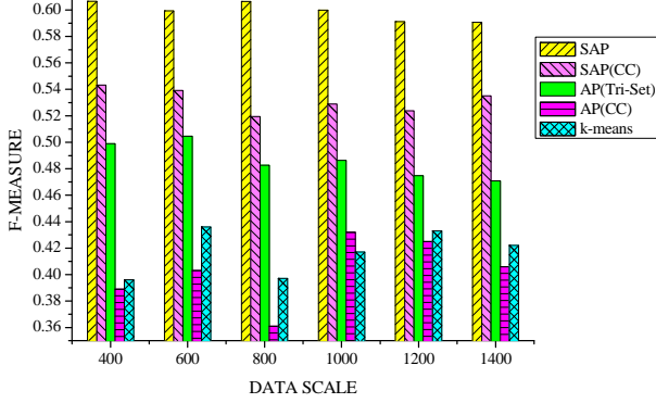
Fig. 2 F-measure comparison
