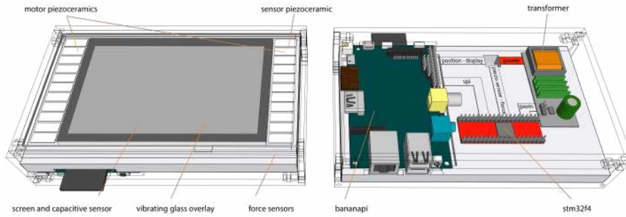
Fig. 2. Device structure.
