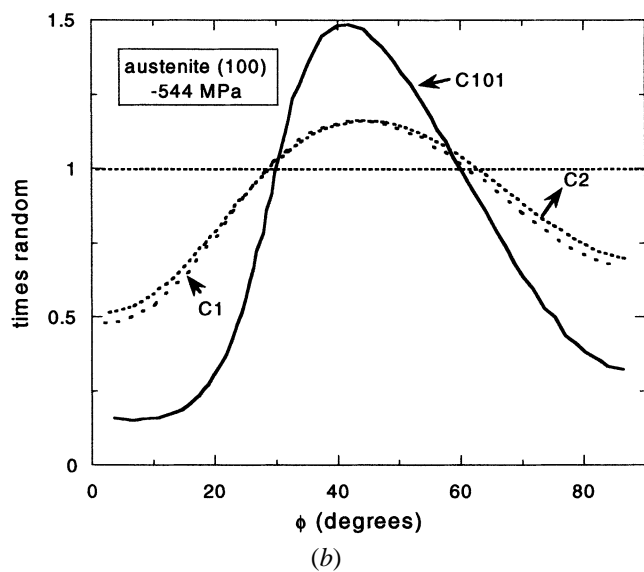
Fig. 9—(100) axial distribution plot for austenite from cycles C1, C2, and C101 during (a) the loading part of the cycle at -715 MPa and (b) the unloading part of the cycle at -544 MPa.
