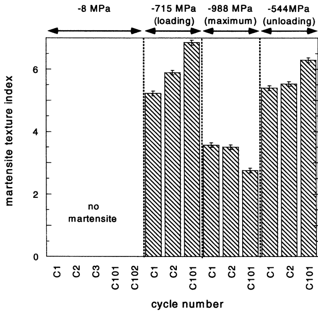
Fig. 7—Martensite texture index at various stresses for the different cycles.
