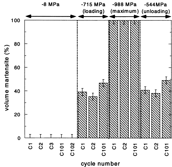
Fig. 5—Volume martensite (pct) at various stresses for the different cycles.
