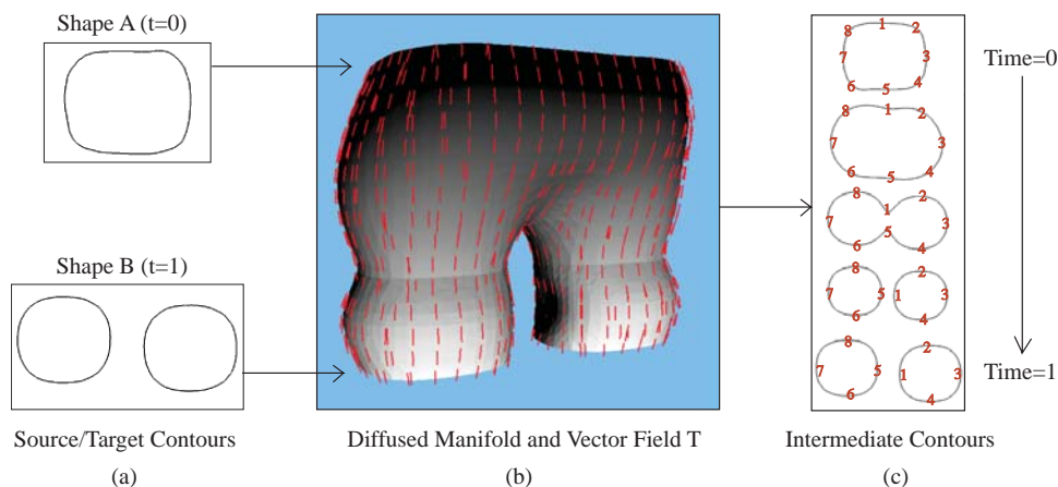
Fig. 2. (a) 2D example of mapping from one closed contour (shape A) to two disjoint contours (shape B). (b) 2D Manifold extracted from the implicit morph spanning 2D space and time. The surface is colored according to the value of the scalar field s . Red lines depict the vector field \mathbf{T} defined by the gradient of s . (c) Propagation of labels along the vector field generates an explicit mapping shown as labeled points on the contours.
