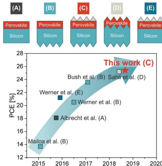
Fig. 1 Different reported texture configurations for experimentally realized perovskite/silicon tandem solar cells including the main developments with the authors and PCE as denoted in the figure. Device schematics indicate where the texture position is located. Device (A) is a fully flat device. Device (B) is a back-side textured device. Device (C) is a back-side textured device with the LM foil as experimentally developed in this work. Device (D) is a both-side textured device whereas device (E) is a fully flat device with the LM foil. If the device has no LM foil, a planar AR coating is considered (not depicted in the schematics for clarity).
