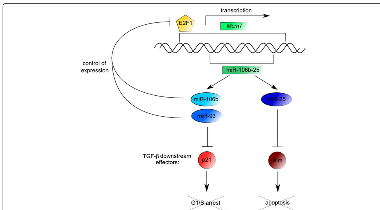
Figure 5 The E2F1/miR-106b-25/p21 pathway. In gastric cancer, miR-106b-25 cluster is activated by E2F1 in parallel with its host gene, Mcm7 . In turn, miR-106b and miR-93 regulate E2F1 expression, establishing a miRNA negative feedback loop. Over-expressed miR-106b, miR-93, and miR-25 inhibit the synthesis of p21 CIP1 and Bim (TGF- \beta downstream effectors) and therefore prevent cell cycle inhibition and apoptosis.
