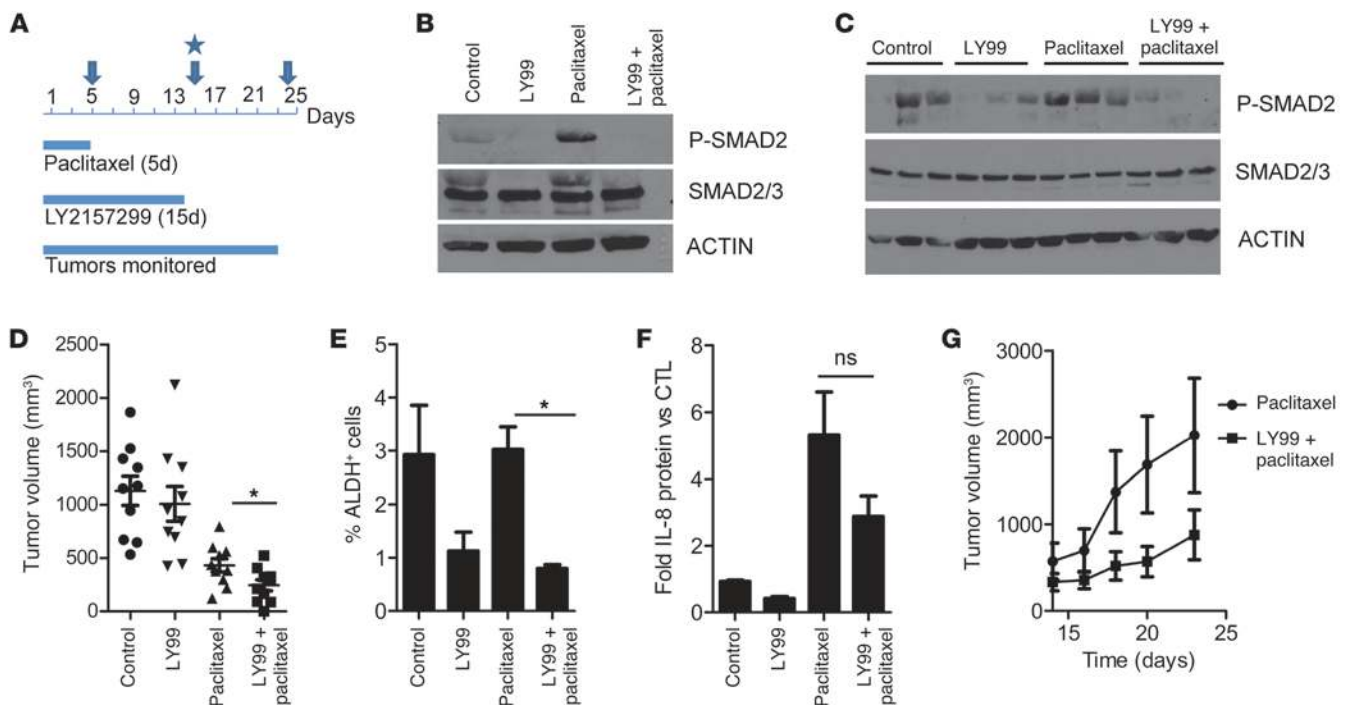
Figure 6 TGF- \beta inhibition in vivo abrogates tumor-initiating potential after chemotherapy. (A–C) Female athymic mice were injected with SUM159 cells in the number 4 mammary fat pad. (A) Once tumors reached a volume of \geq 75 mm 3 , mice were randomized to 4 treatment groups ( n = 10 mice per group): (a) vehicle (control), (b) LY2157299 (100 mg/kg/p.o. twice daily), (c) paclitaxel (20 mg/kg/d i.p. 5 times), and (d) both drugs. The arrow at day 5 represents the cessation of paclitaxel treatment. The arrow and star at day 15 indicate the cessation of LY2157299 treatment and the procurement of xenografts, respectively. The arrow at day 23 represents the cessation of monitoring for tumor growth. Lysates from xenografts harvested after (B) 5 days and (C) 14 days were assessed for total SMAD2/3 and P-SMAD2 levels by immunoblot analysis. (D) Tumor volumes calculated on day 14 ( *P = 0.035 ; Mann-Whitney). Symbols indicate individual tumors; horizontal bars represent the mean. (E) Single cell suspensions derived from xenografts harvested on day 14 were analyzed for ALDH activity using the ALDEFUOR assay ( *P = 0.002 ). (F) Serum was collected from mice at the time of tumor harvesting and sacrifice and analyzed for IL-8 protein levels by ELISA. Each bar represents mean IL-8 levels over control \pm SEM ( n = 3 ). ns, not significant. (G) Progression of tumor volumes during days 14–23 in mice treated with paclitaxel with or without LY2157299 during days 1–14 ( n = 5 ). Tumors treated with vehicle (controls) or LY2157299 alone are not included, as they had reached a volume of \geq 1 cm 3 on day 14 (start of x axis). Because of the large tumor burden, these mice had to be sacrificed as per institutional guidelines. Error bars indicate SEM.
