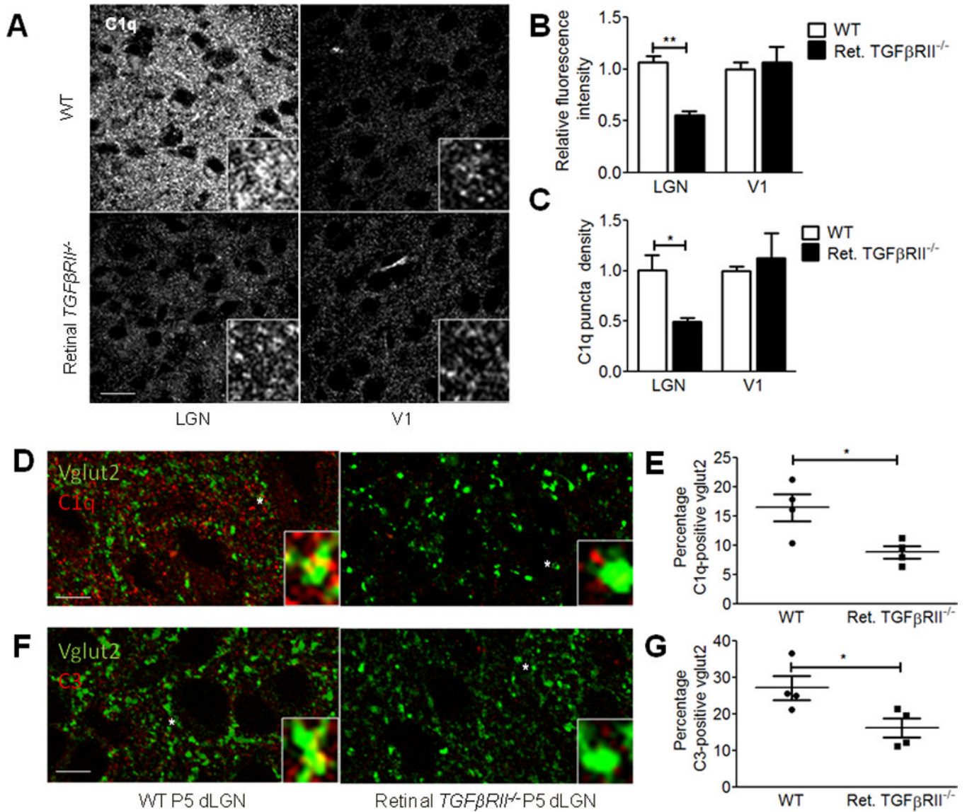
Figure 5. Retinal TGF-β signaling is required for complement localization in the dLGN (A) C1q immunohistochemistry in the dLGN and primary visual cortex (V1) shows reduced C1q fluorescence intensity in the dLGN but not in V1. Scale bar = 20μm. Inset shows 3× magnification. (B) Quantifying relative fluorescence intensity showed significant reduced intensity in the dLGN of retinal TGFβRII -/- vs. WT mice (two-way ANOVA, n=4 mice/group, **p<0.01, F(1,12)=11.21). No differences were observed in V1. (C) C1q puncta density quantification showed significantly reduced C1q puncta density in the dLGN in retinal TGFβRII -/- mice vs. WT littermates (two-way ANOVA, n=4 d C1q expression. Microglia acutely isolated using CD45 immunopanning showed no significant difference in C1q levels (two-way ANOVA, n= 5 mice/group, *p<0.05, F(1,8)=7.48). No difference in C1q puncta density was observed in V1. (D) C1q localization to vglut2-positive RGC terminals is reduced in the retinal TGFβRII -/- mouse. Immunostaining for C1q and vglut2 in WT and retinal TGFβRII -/- P5 dLGNs showed a reduction in co-localization of C1q and vglut2. Scale bar = 20μm. Star indicates the enlarged synaptic puncta shown in the inset. (E) Quantification of C1q co-localization with vglut2 showed significantly reduced synaptic localization of C1q in retinal TGFβRII -/- mice. Co-localized puncta were identified and
