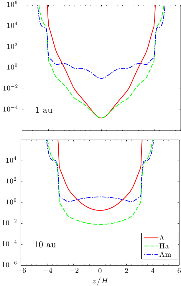
Fig. 2. Ohmic ( \Lambda ; Eq. (15)), Hall ( \text{Ha} ; Eq. (16)), and ambipolar ( \text{Am} ; Eq. (17)) Elsasser numbers in the initial state versus height z at 1 au (top) and 10 au (bottom), assuming a constant vertical magnetic field with \beta_0 = 10^5 .
