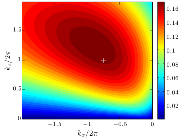
Fig. B.2. Growth rate of the ambipolar-MRI for B_{z0} = 0.025 and B_{y0} = 0.1 as a function of the horizontal and vertical wavenumbers, k_x and k_z . The largest growth rate available in the simulation obtains for (k_x, k_z) = 2\pi \times (-0.75, 1) (white cross).
