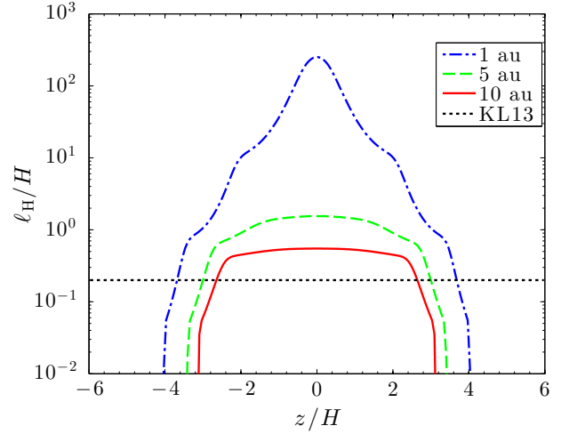
Fig. 3. Hall lengthscale \ell_H (Eq. (18)) versus height z at 1, 5, and 10 au. The dotted line denotes the threshold above which saturation via zonal magnetic fields occurs in unstratified simulations with net vertical magnetic flux (KL13).
