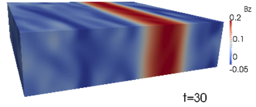
Fig. A.2. Snapshot of B_z in our unstratified Hall-MRI run at t = 30 . The flow exhibits a zonal-field structure similar to that discovered by KL13.
